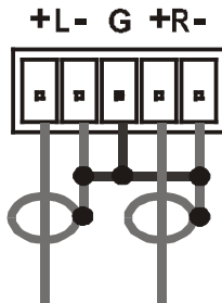
Figure 6: Connecting the Unbalanced Stereo Audio Input
