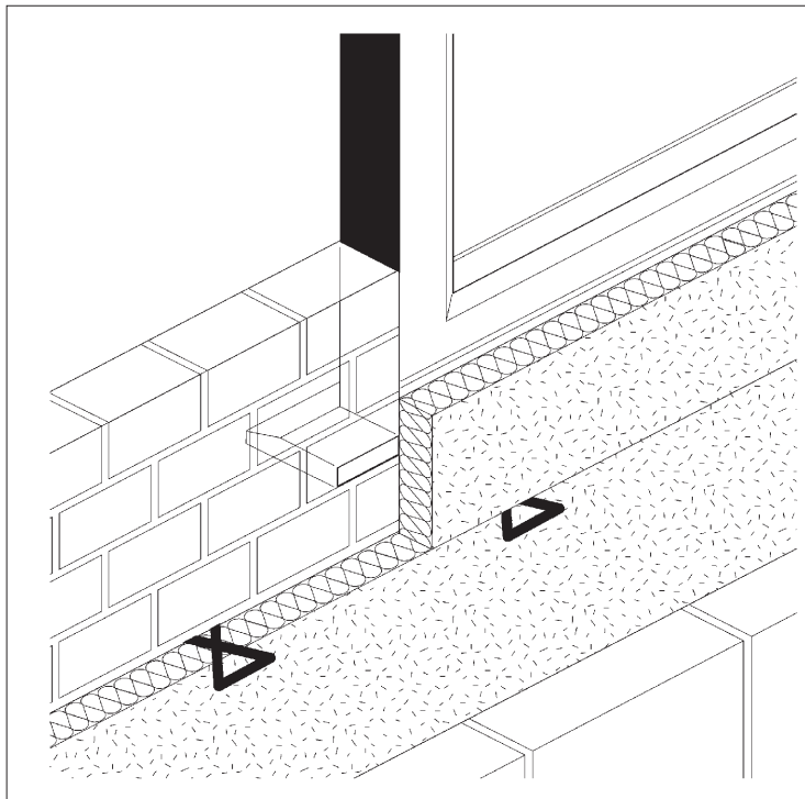
Figure 5 Use of cut pieces
