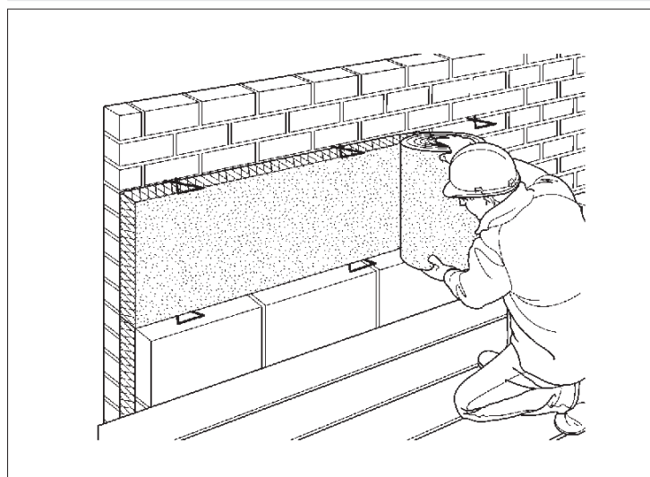
Figure 2 Installation of rolls between upper and lower wall ties
