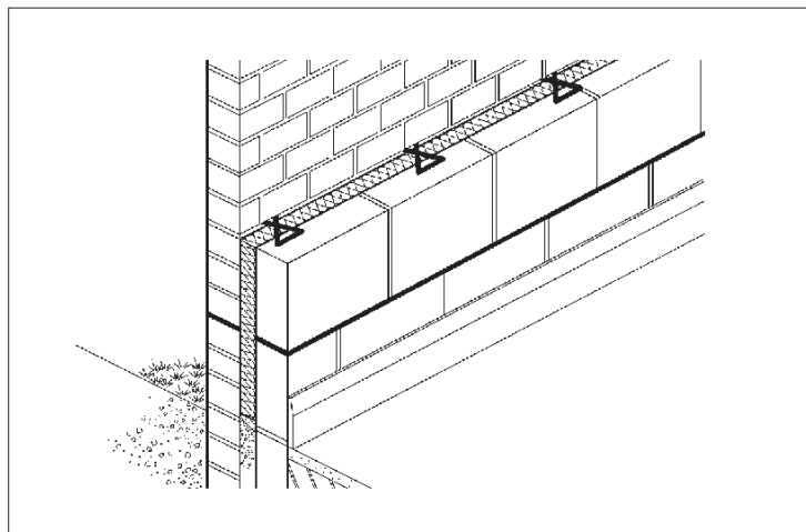
Figure 1 First run of roll below the DPC
