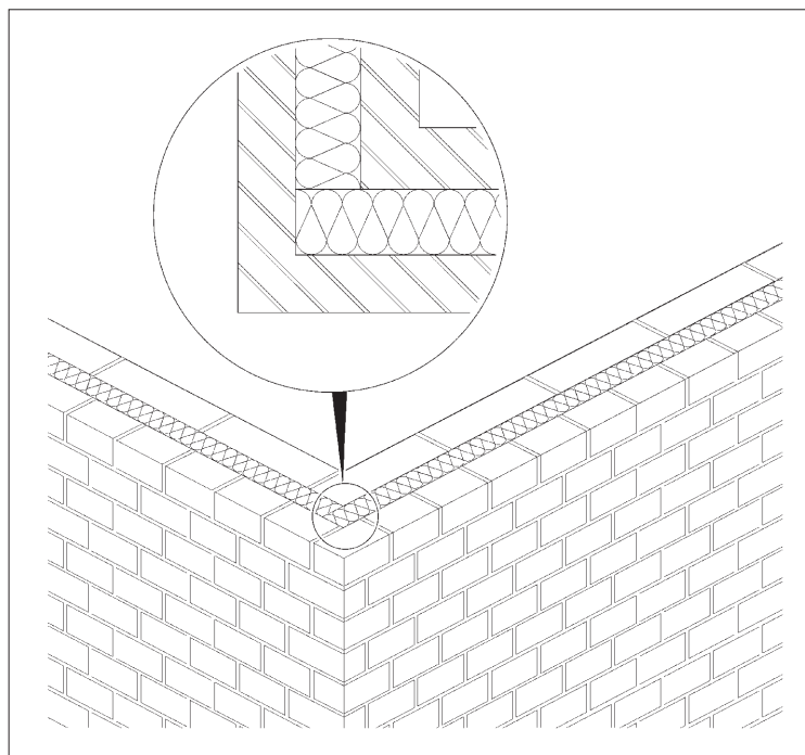
Figure 4 Rolls close butt jointed at corners
