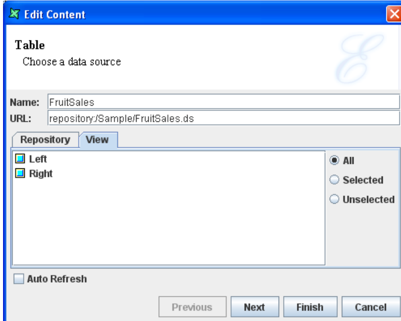
Figure 2.2. Dynamic Datasource
