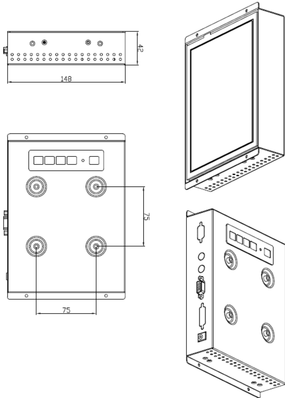
Figure 1.1: Dimensions of OPD-1086B
