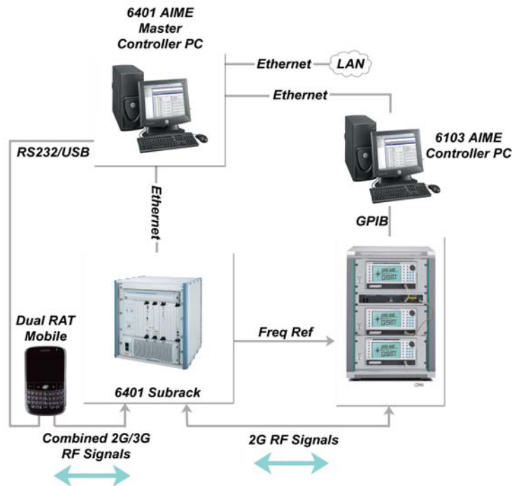
Intersystem Handover (ISHO) Test Solution
