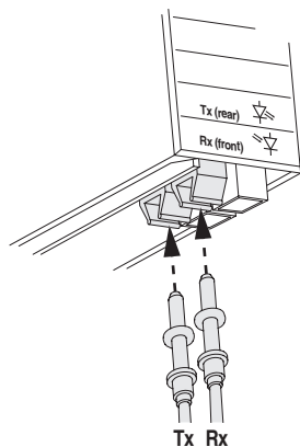
Figure 4.1 SynchLink Connections
