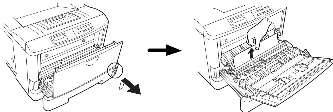
Figure 5.4. Registration Roller
