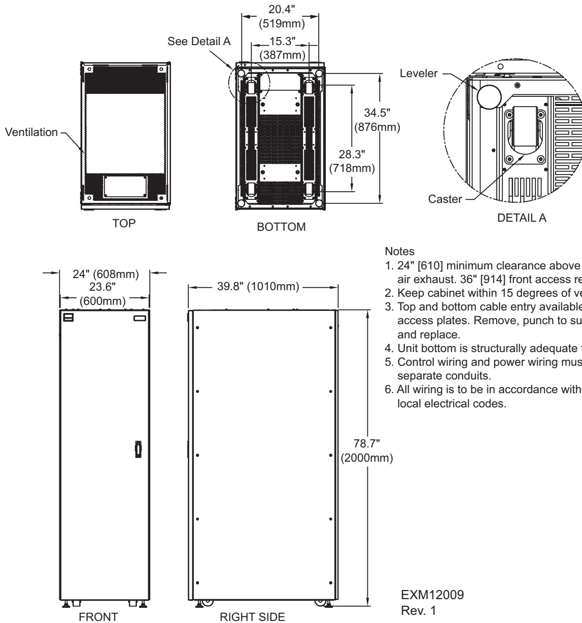
Figure 9 Outline drawing, Liebert eXM TXC for Liebert eXM, 10-100kVA
