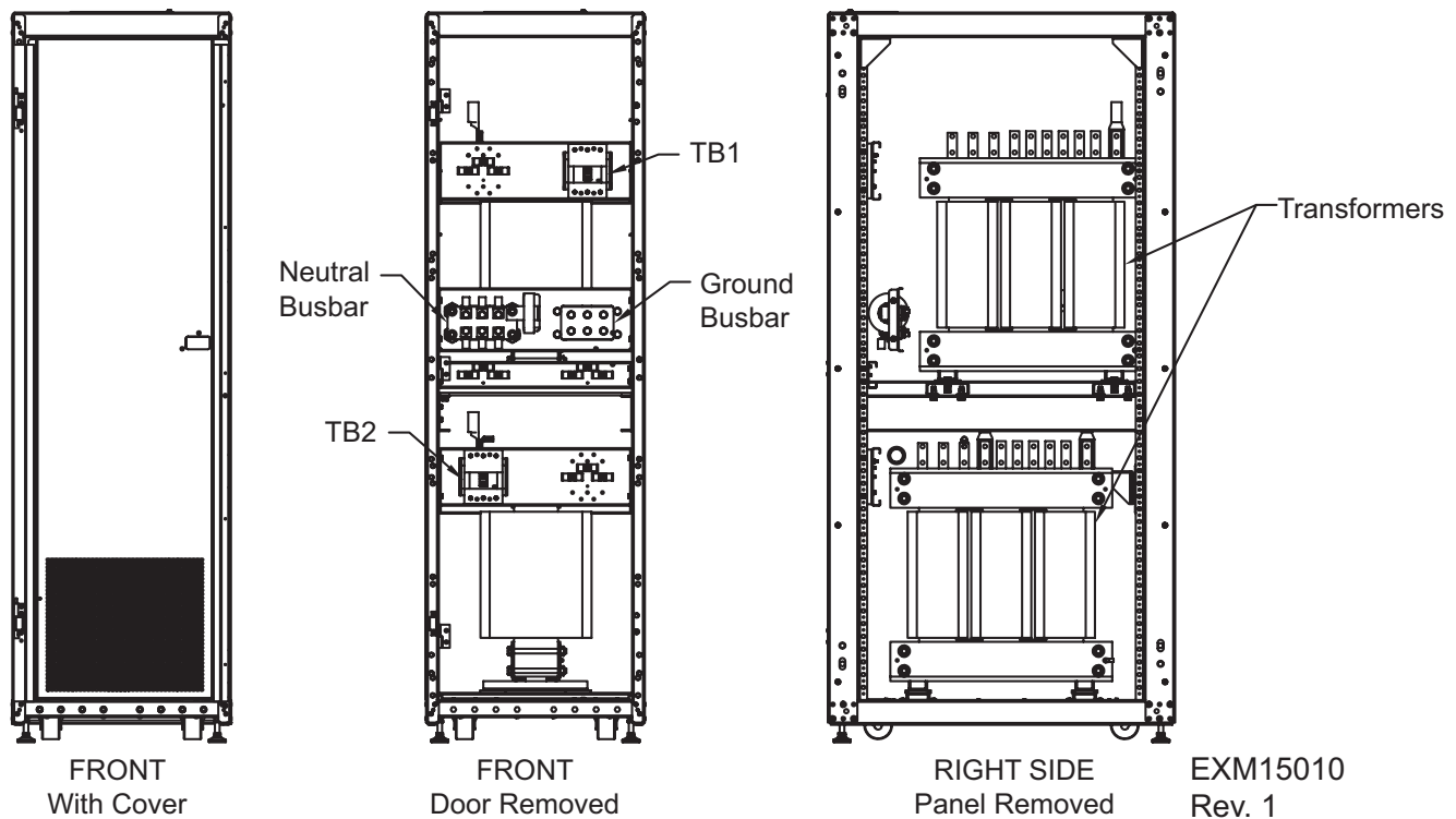
Figure 7 Busbars—Liebert eXM TXC
