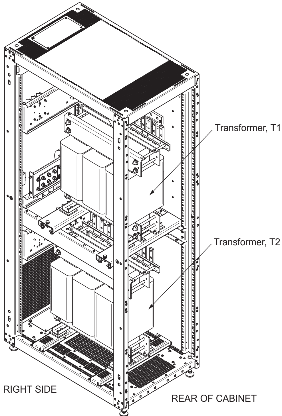
Figure 10 Liebert eXM TXC transformer location
