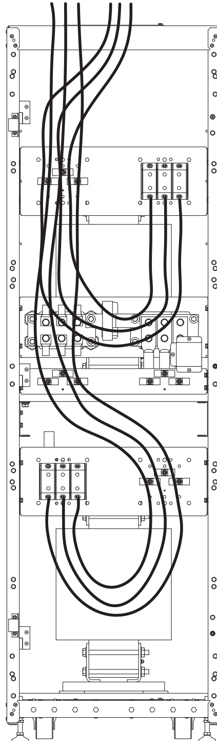
Figure 11 Bend radius - Top feed power connections, 10-100kVA system
