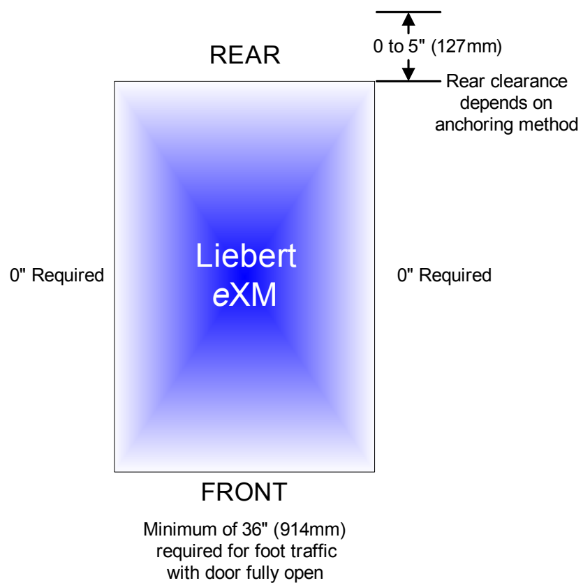
Figure 5 Clearances—Front, side and rear
