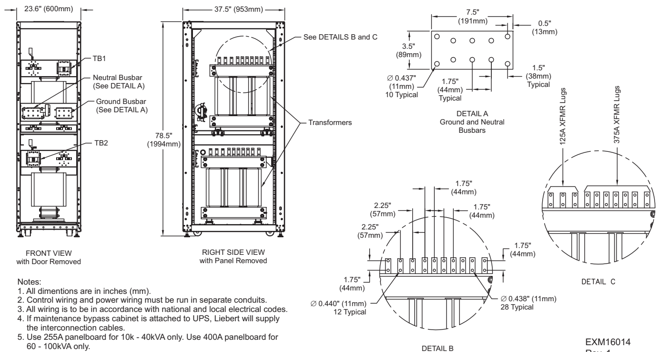
Figure 7 Busbars—Liebert eXM TXC
