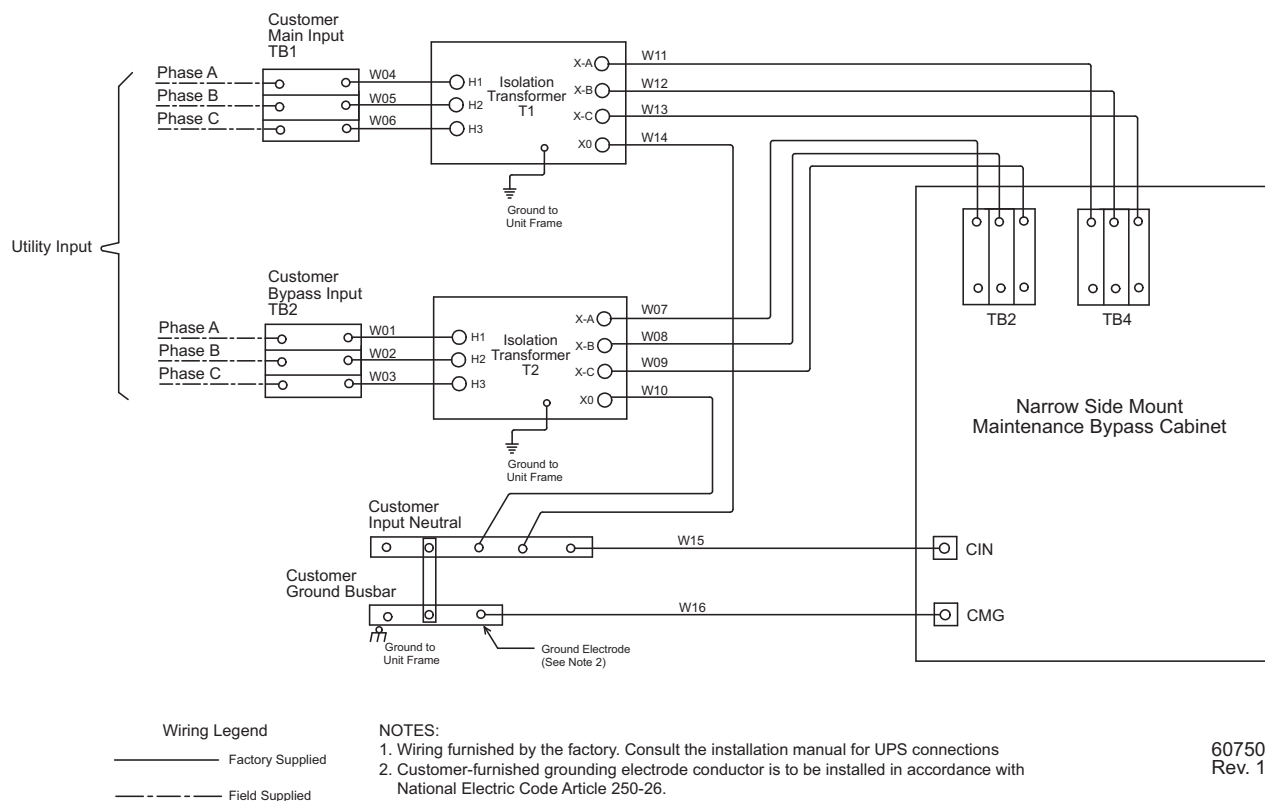
Figure 2 Schematic - Liebert eXM TXC to Maintenance Bypass Cabinet
