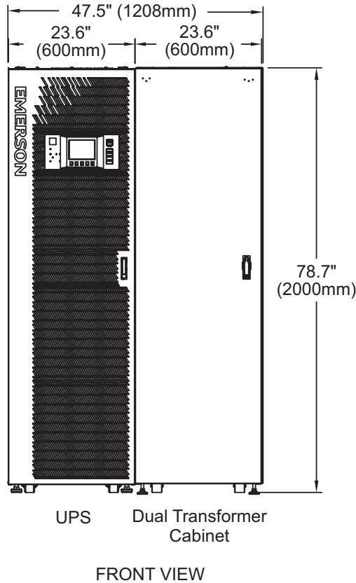
Figure 8 Lineup arrangement, Liebert eXM with Liebert eXM TXC
