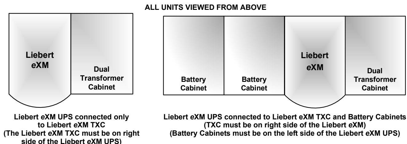
Figure 4 Cabinet arrangement
