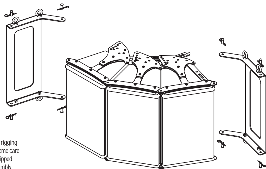
GEO S830s with hardware for horizontal rigging.
