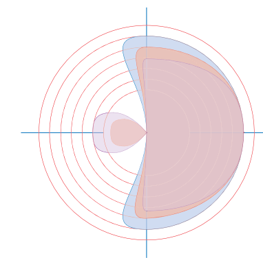
Fig 3: Cardioid sub-bass coverage from CD SubBass
