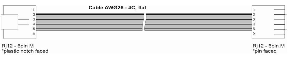
Figure 4: Interconnection cable ICM-X
