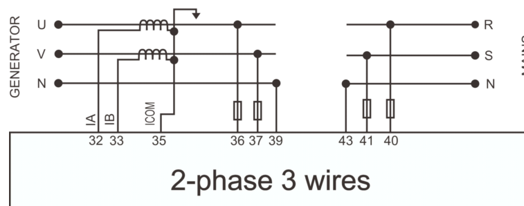
Two-phase three-wire connection wiring diagram (to LXC9220 example)
