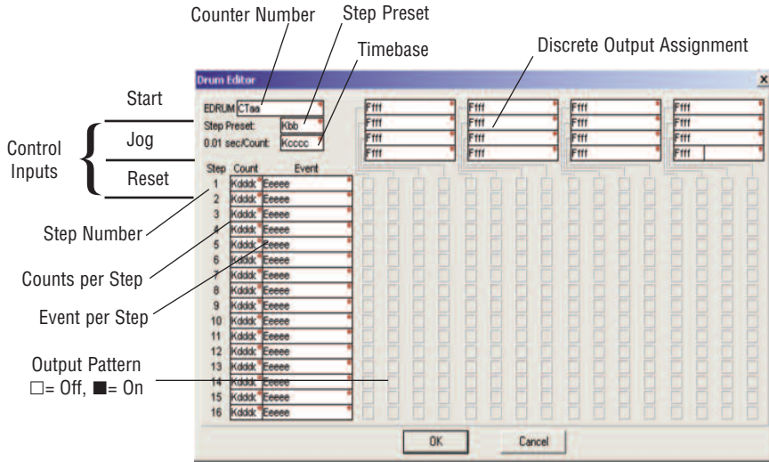
DirectSOFT 5 Display
