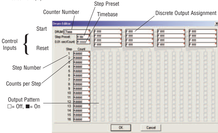
DirectSOFT 5 Display
