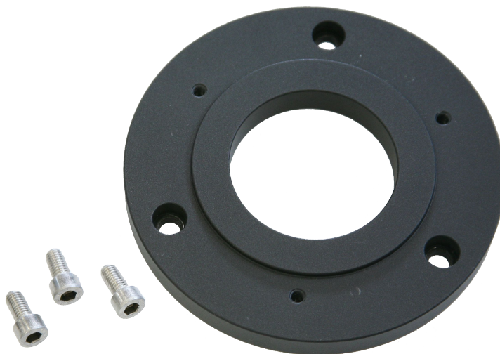
Fig. 4.8: Optional tripod adapter and screws.
