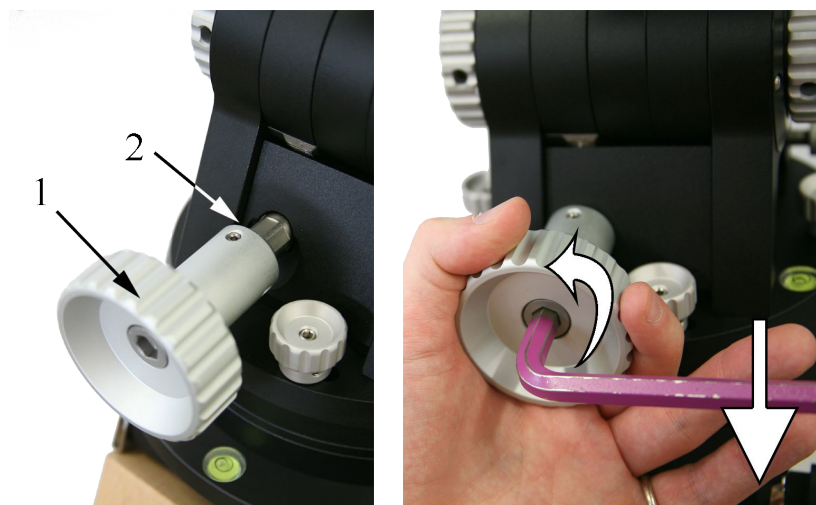
Fig. 4.12: Assembling the altitude adjustment knob.
