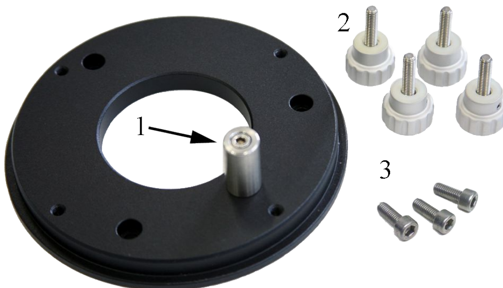
Fig. 4.6: Base adapter assembly and mount locking knobs.
