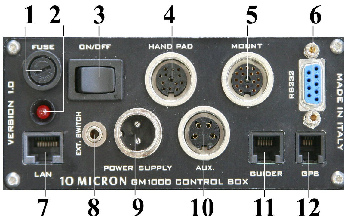
Fig. 5.1: The connection panel on the control box.
