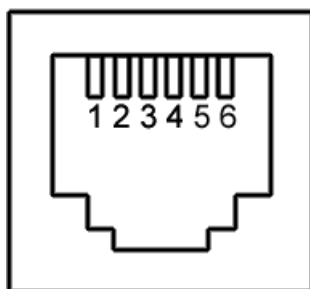
Fig. 5.6: Autoguider port pinout.
