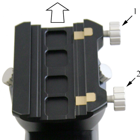
Fig. 4.18: The double-sized dovetail.
