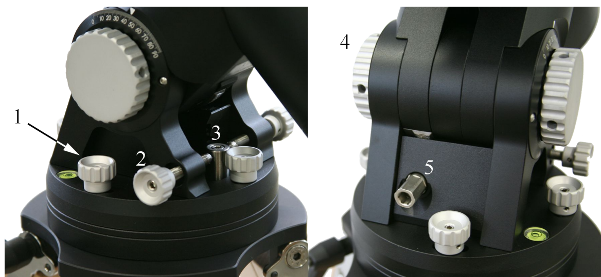
Fig. 4.19: Fine altitude and azimuth adjustment system.
