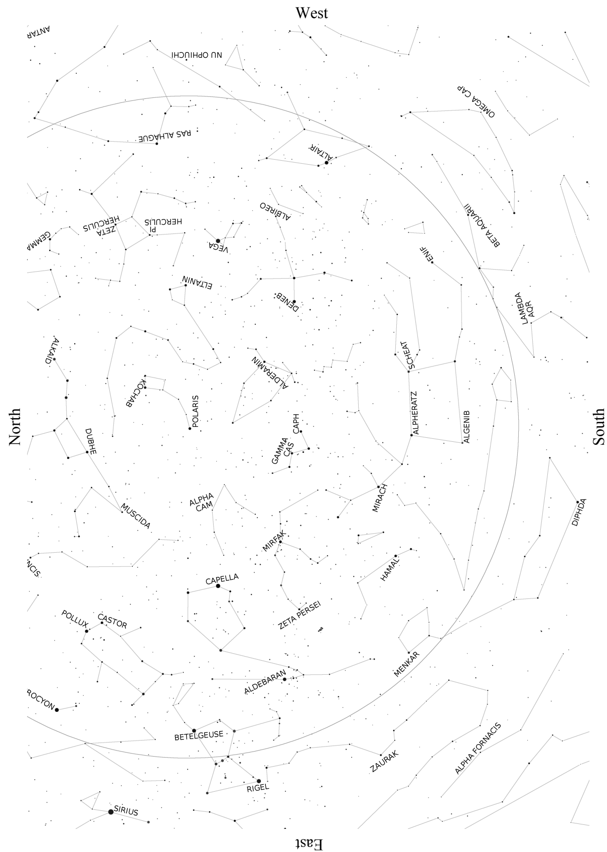
Northern Hemisphere Chart – December to February
