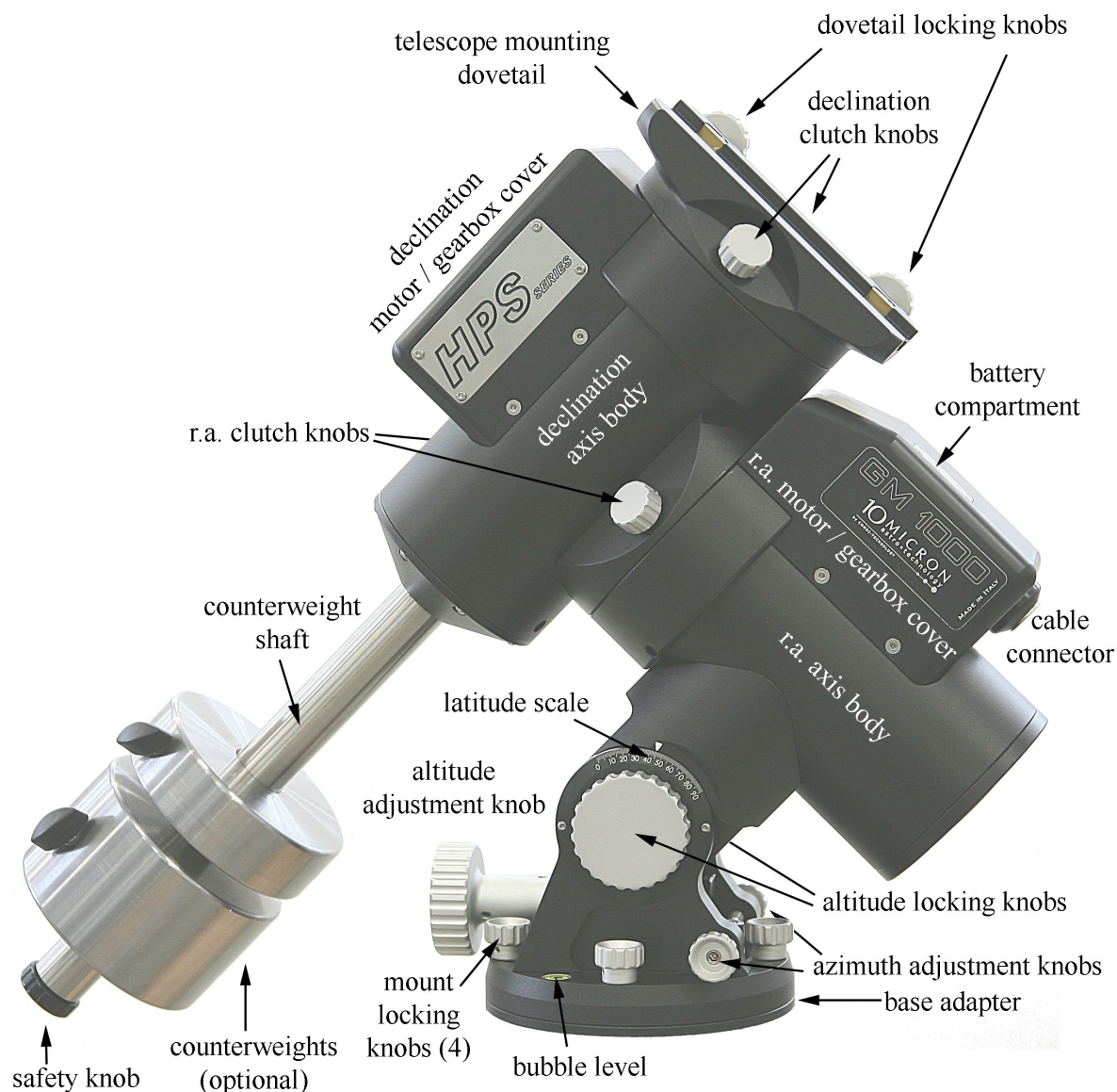
Fig. 4.5: GM1000HPS mount parts.
