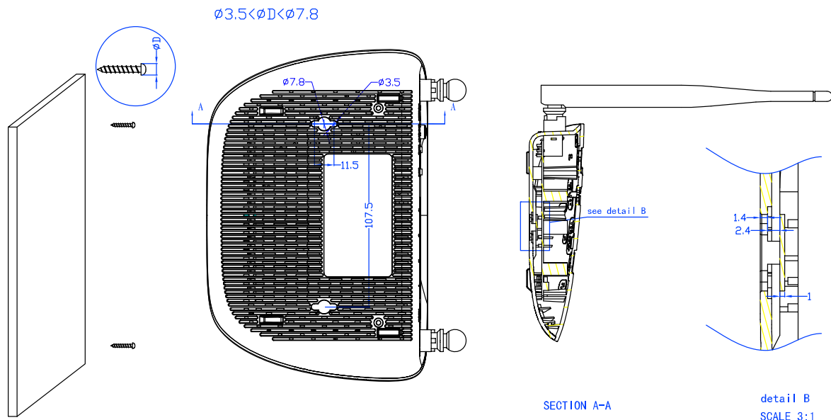
Figure 2-3 Wall-mount Install
