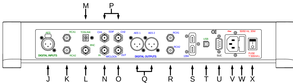
Figure 7 – Rear panel
