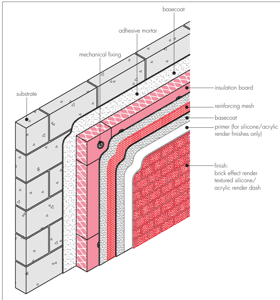
Figure 1 Climatherm Mineral Wool External Wall Insulation System
