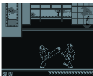
Figure 11.45.: ZXBox
