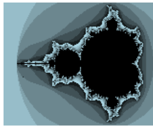
Figure 11.33.: Fractals: Mandelbrot set
