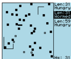
Figure 11.27.: Wormlet game
