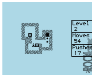
Figure 11.22.: Sokoban
