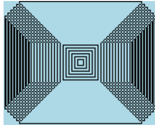
Figure 11.34.: Mosaique
