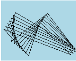
Figure 11.31.: Demystify
