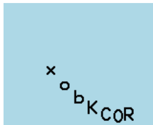
Figure 11.29.: Bounce
