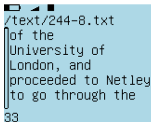
Figure 11.42.: Text Viewer
