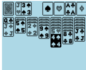
Figure 11.23.: Klondike solitaire
