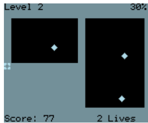
Figure 11.28.: Xbox
