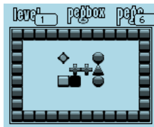
Figure 11.15.: pegbox
