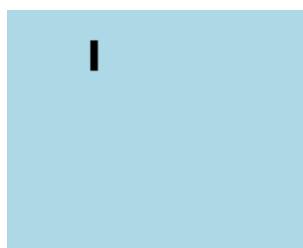
Figure 11.20.: Snake
