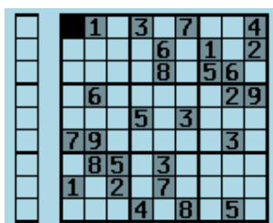
Figure 11.26.: Sudoku
