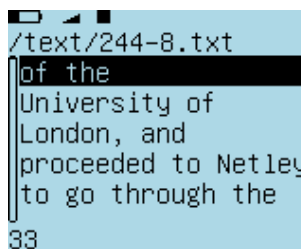
Figure 11.44.: A bookmark
