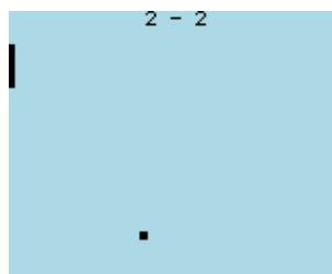
Figure 11.16.: Pong
