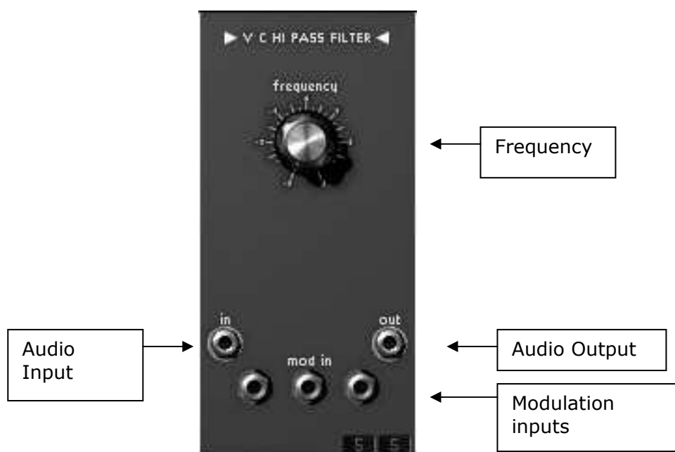
High-pass filter 24dB
