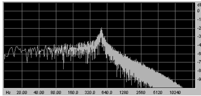
Low Pass 12 dB/Octave
