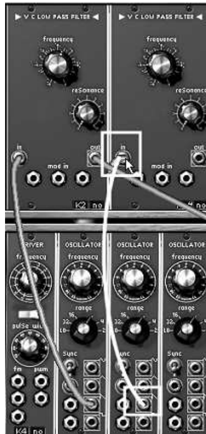
Connection between oscillator 2 and filter2
