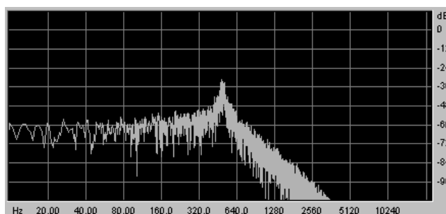
Low Pass 24 dB/Octave Filter
