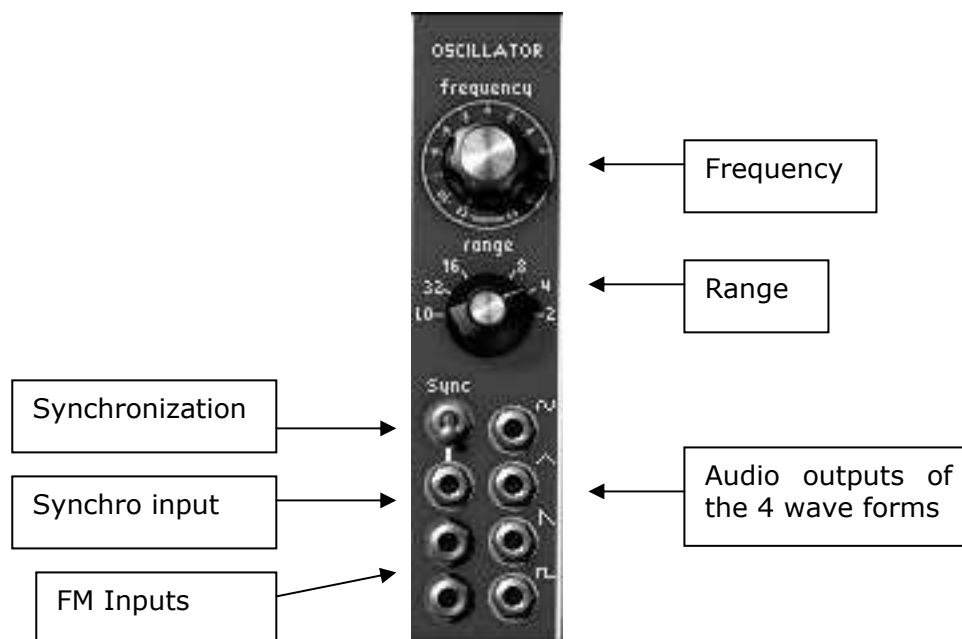
Oscillator 921b
