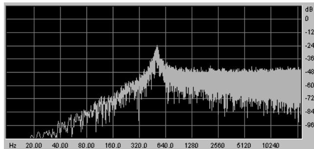
High Pass 12 dB/Octave
