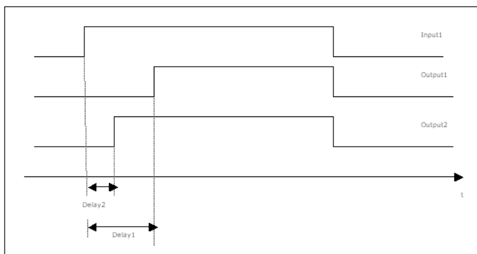
Parallel mode
