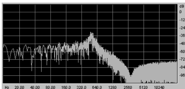
Low shelf 12 dB/Octave
