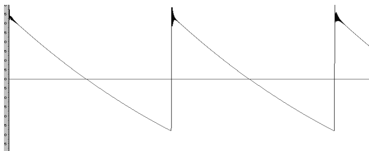
Temporal representation of a waveform on a Modular Moog 55
