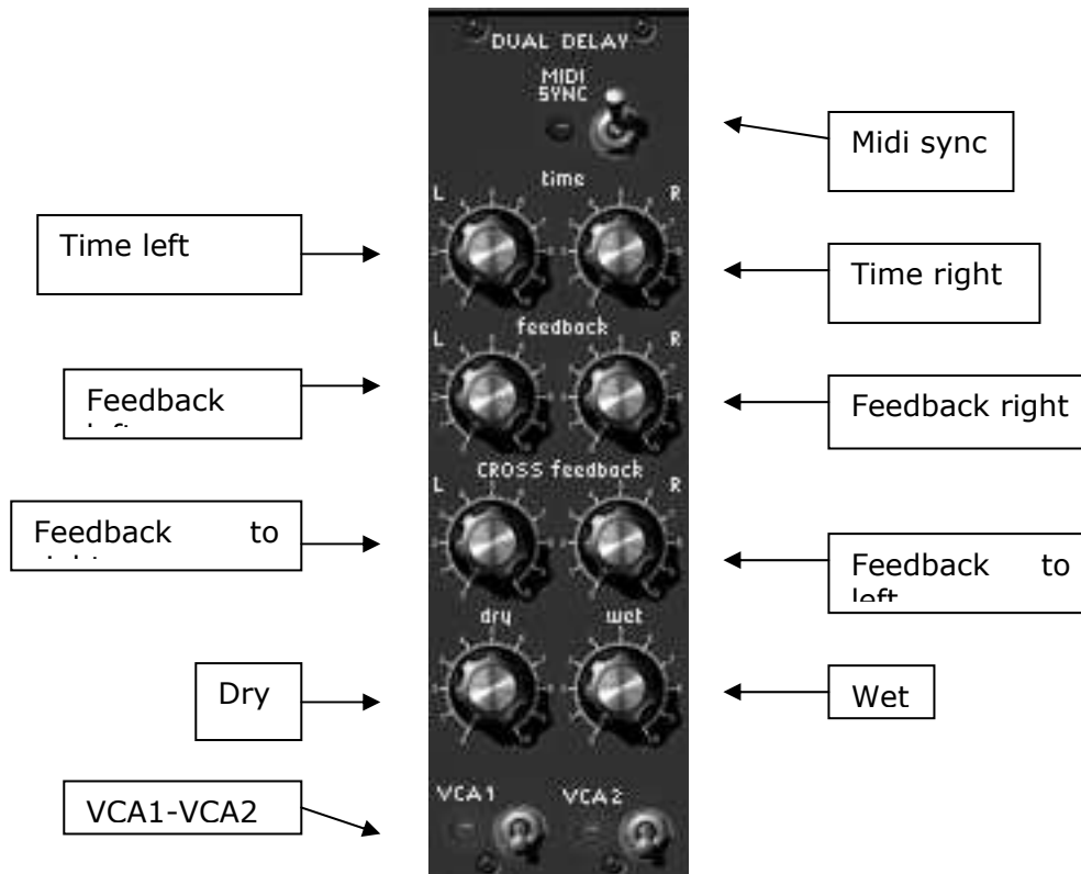
Stereo Delay module
