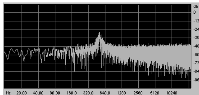
Bell 12 dB/Octave
