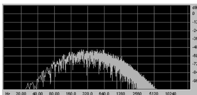
Band Pass 24 dB/Octave
