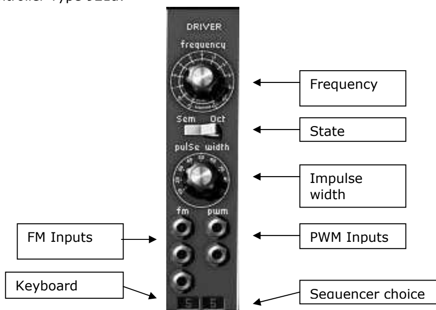
Oscillator 921a
