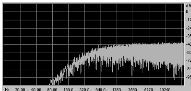
High Pass 24 dB/Octave
