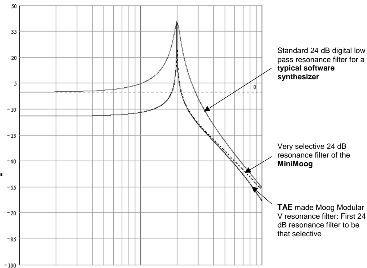
Comparative response filters
