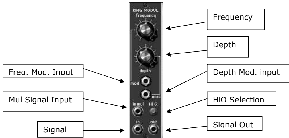
Ring modulator
