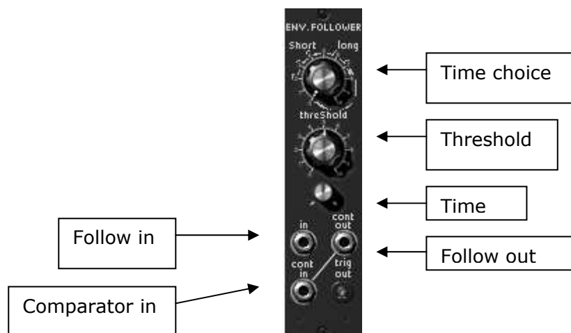
Envelope follower
