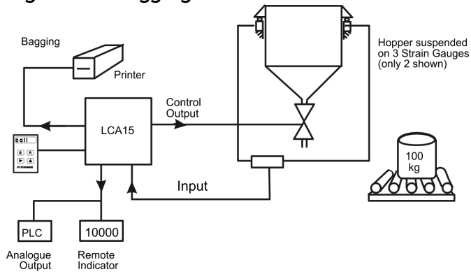
Figure 1.1 Bagging
