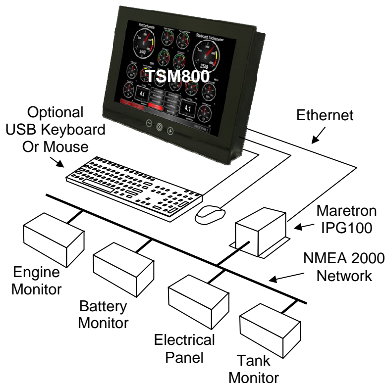
Figure 1 – TSM800 Network Diagram
