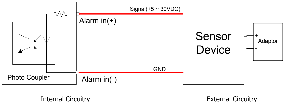
Figure 2-5. Connecting to Alarm Input
