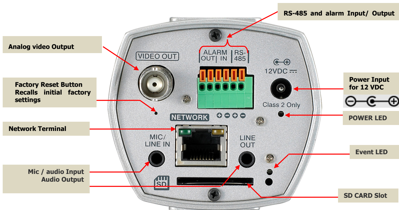
Figure 2-2. IP Camera Rear view
