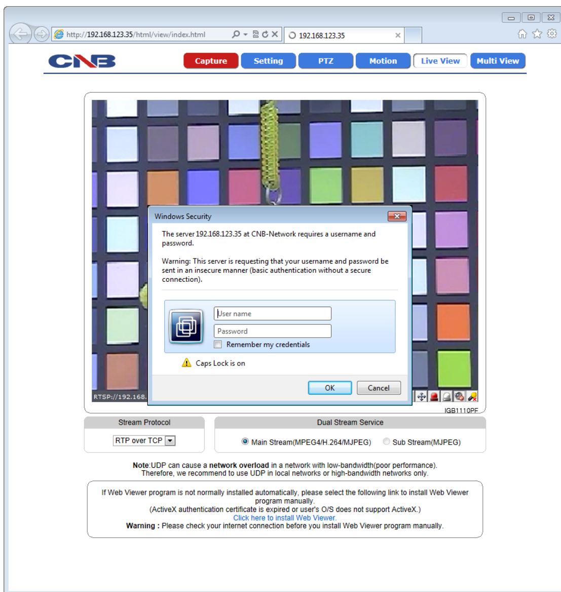
Figure 4-1. Log-in Box
