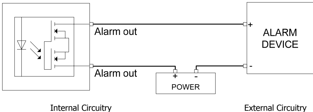
Figure 2-6. Connecting to Alarm Output
