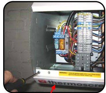
access panel
