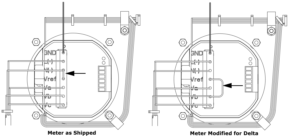
Figure 3.4: Wiring as Shipped, and Modified for Delta
