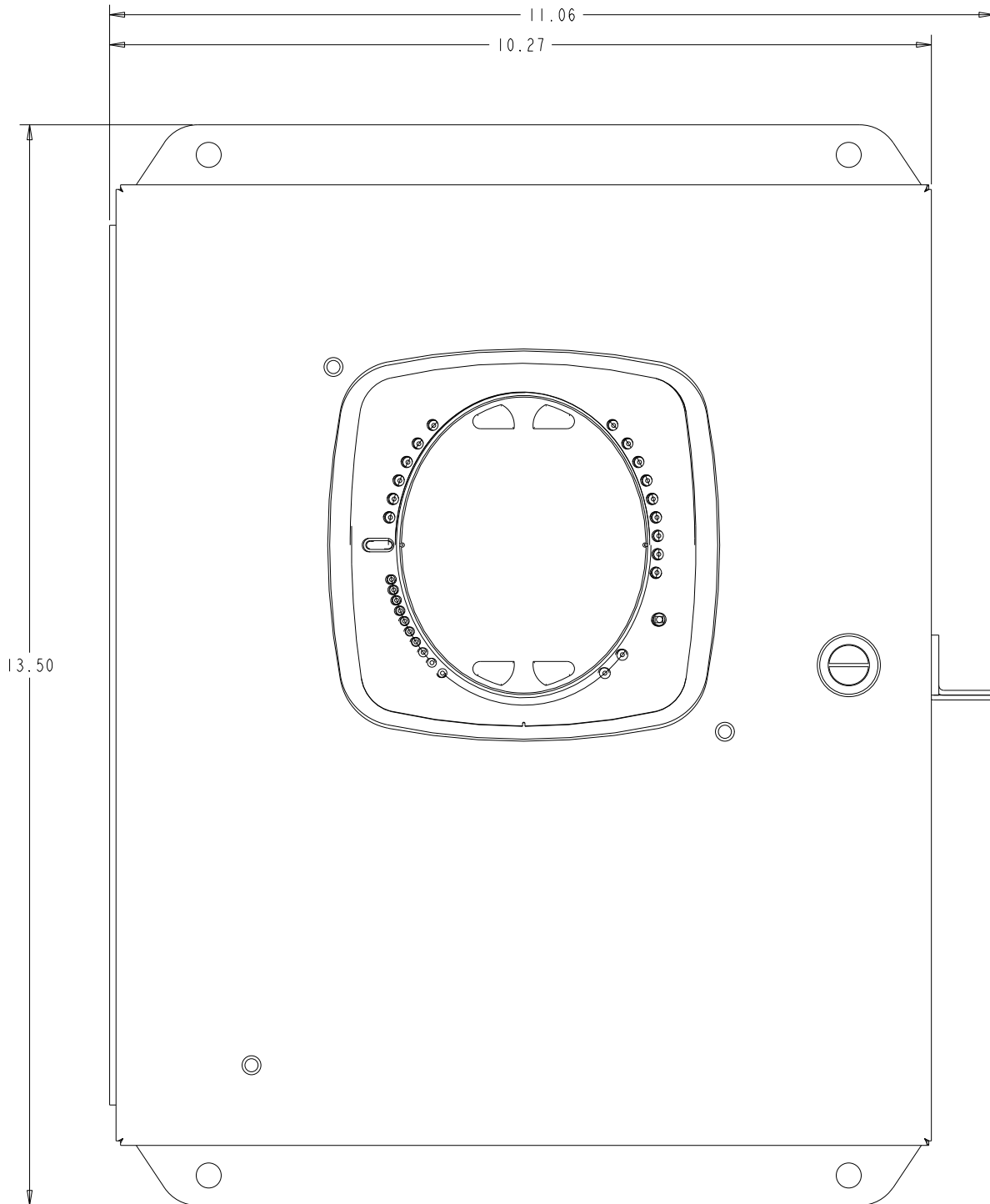
Figure 2.5: Enclosure Front Dimensions
