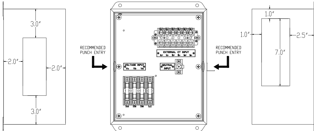
Figure 2.3: Location of Recommended Punch Entries
