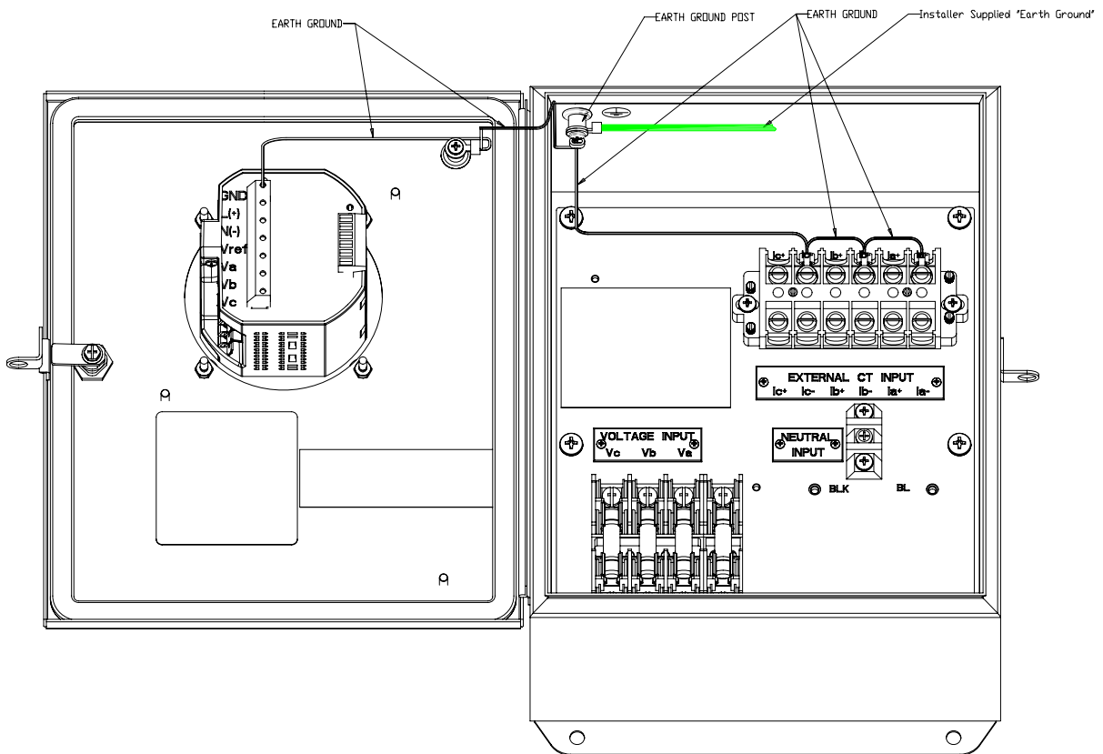
Figure 3.1: Earth Ground Connection
