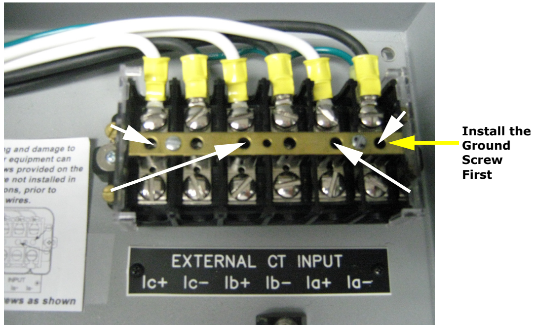
Figure 5.2: Shorting the CTs
