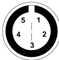
Female 5-pins connector pin out (external view)
