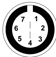
Female 7-pins connector pin out (external view)
