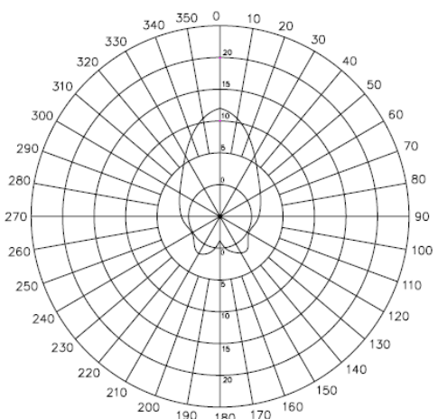
E-Plane Field Patterns for 2.4GHz
