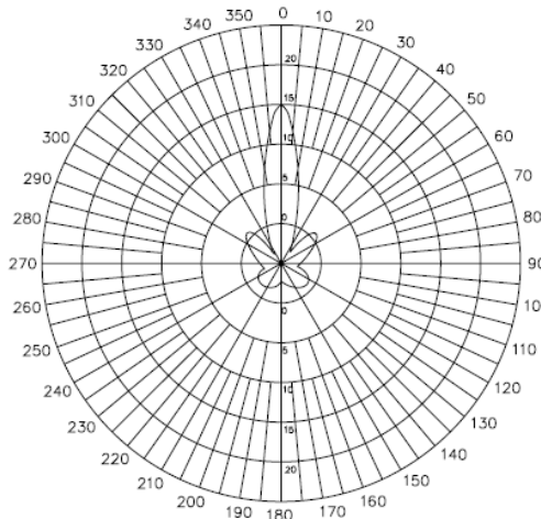
E-Plane Field Patterns for 5.8GHz
