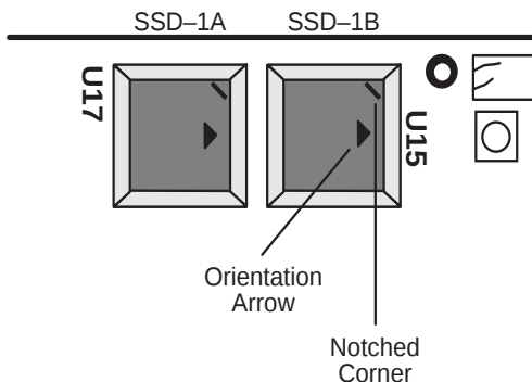
Figure 3-1 PLCC Orientation
