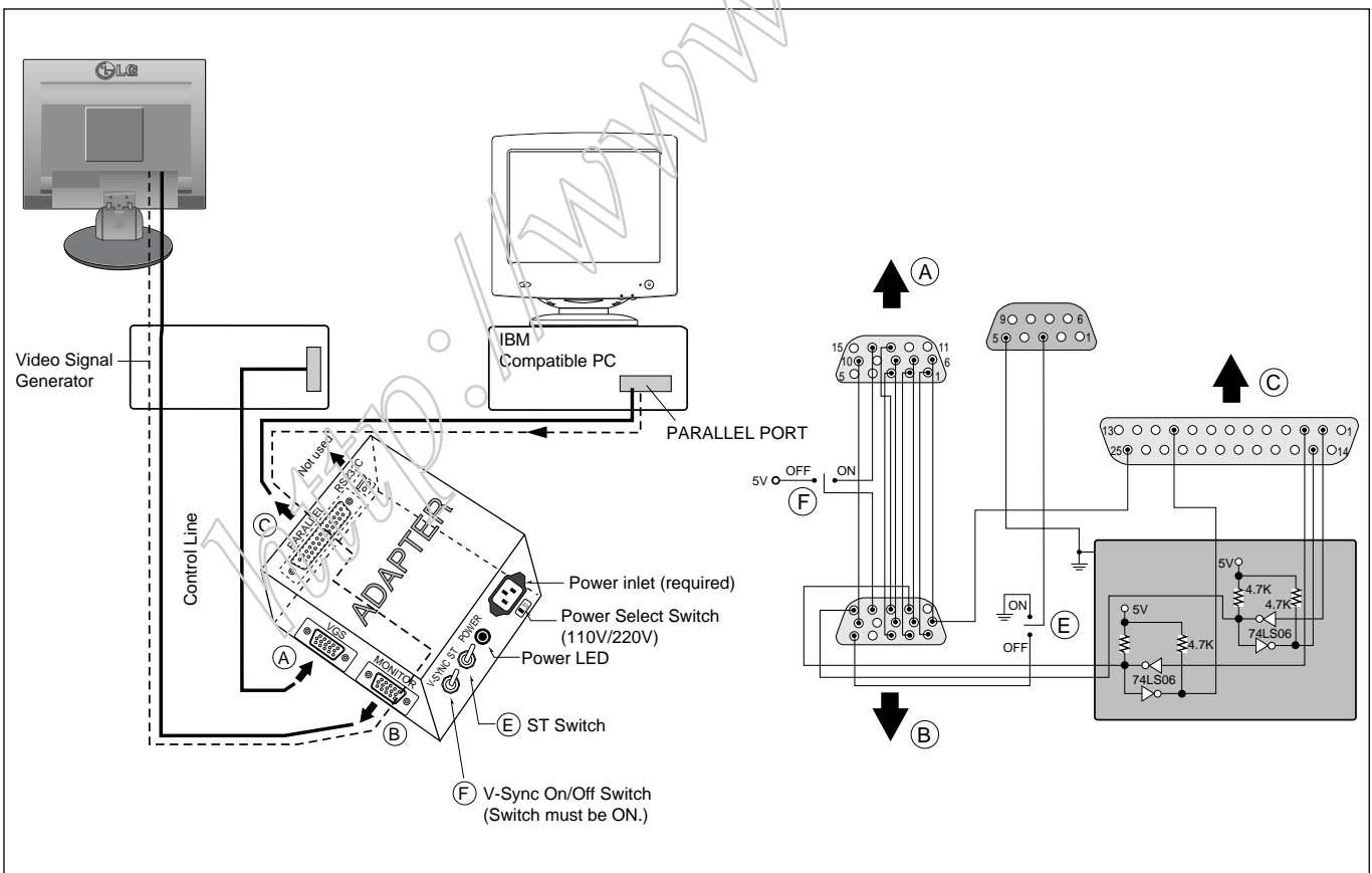
Figure 1. Cable Connection
