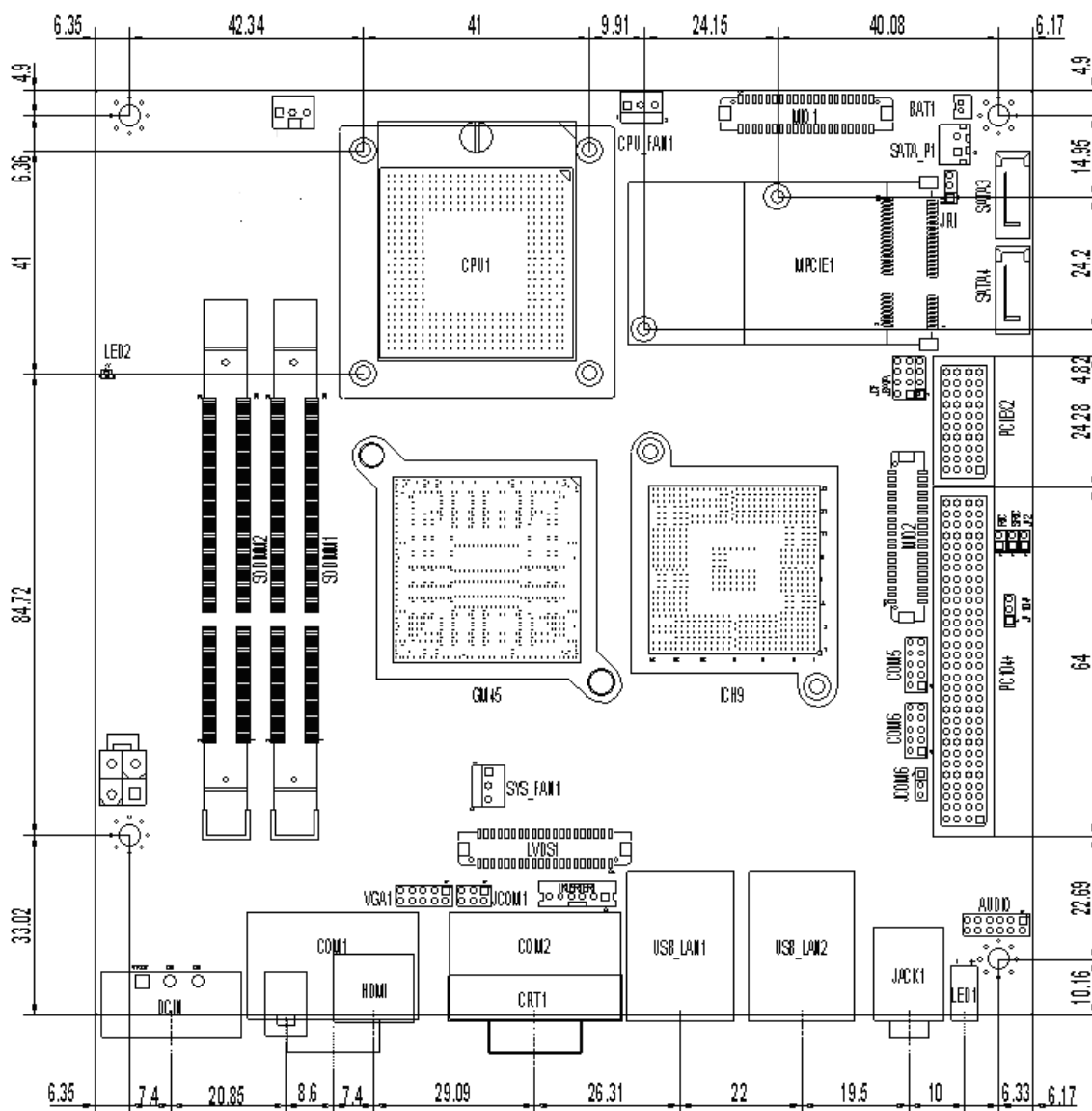
Figure 2.1: Mainboard Dimensions
