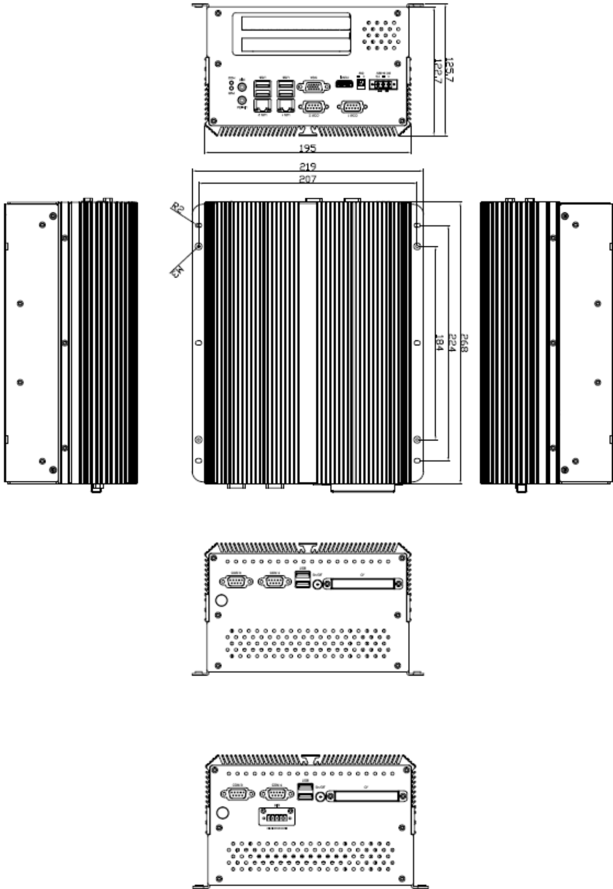
Figure 1.1: Dimensions of the ACS-2675C
