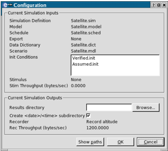
Figure 11.13: Sample Configuration
