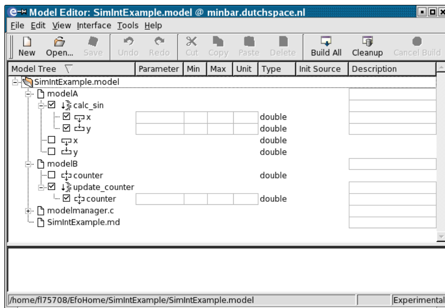
Figure 22.1: Model Editor
