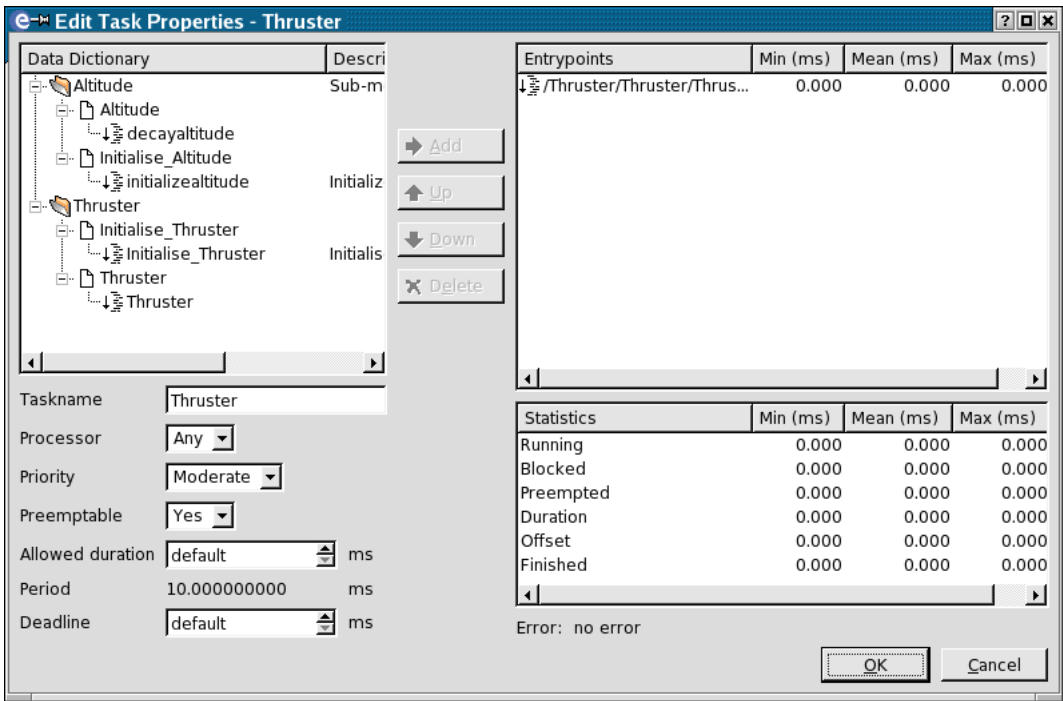
Figure 10.2: Task dialog
