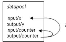
Figure 22.7: Parameter exchange
