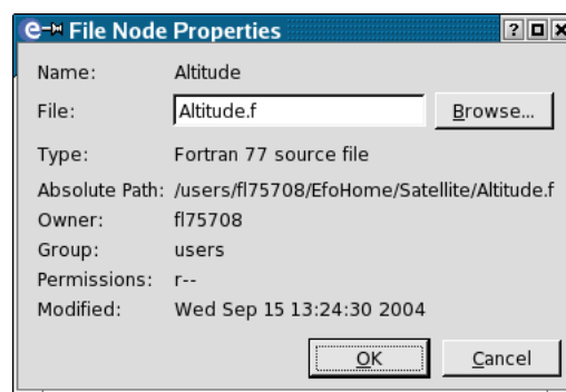
Figure 6.2: File Properties
