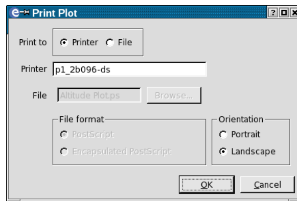
Figure 12.3: Printing plots.
