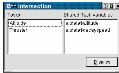
Figure 10.10: Intersection Dialog
