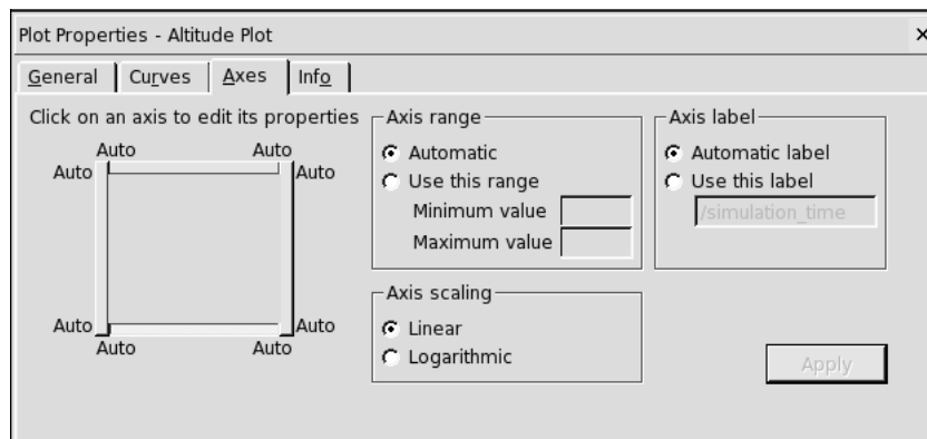
Figure 12.6: Axes properties.
