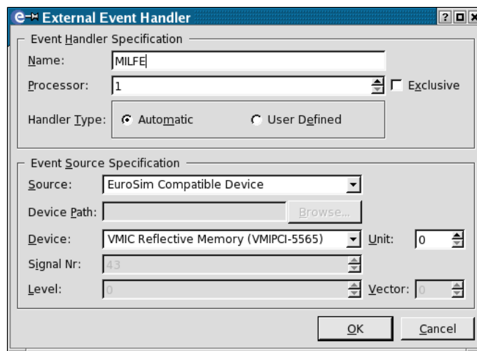
Figure 10.9: External Event Handler Dialog
