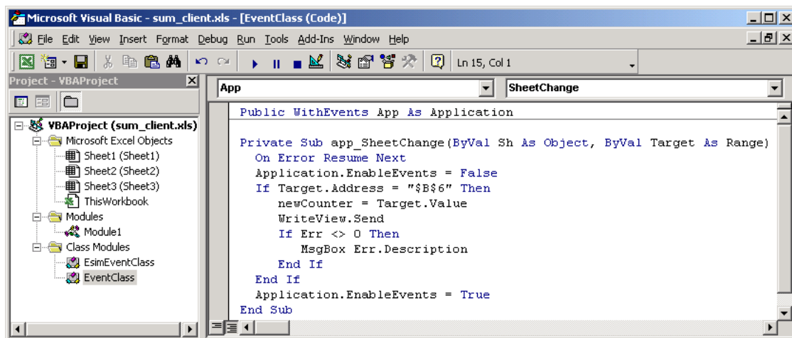
Figure 24.7: The application event handler
