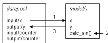
Figure 22.5: Datapool exchanges and update for model A
