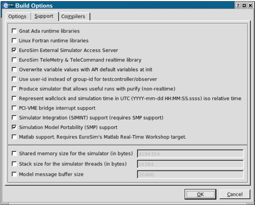
Figure 17.1: Model Editor Build Options dialog box with SMP support enabled.
