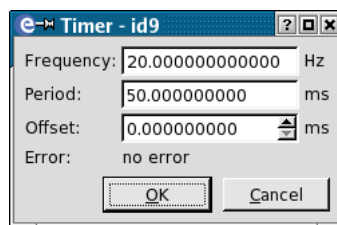
Figure 10.7: Timer Dialog
