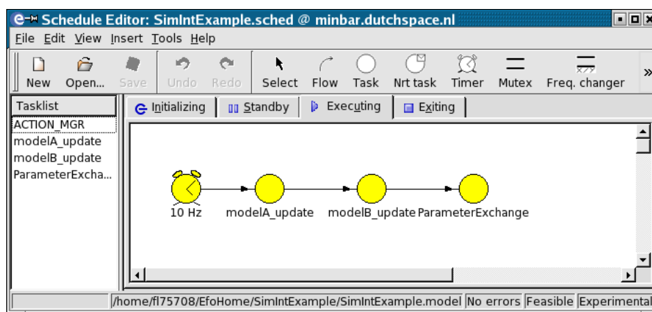
Figure 22.4: Schedule Editor
