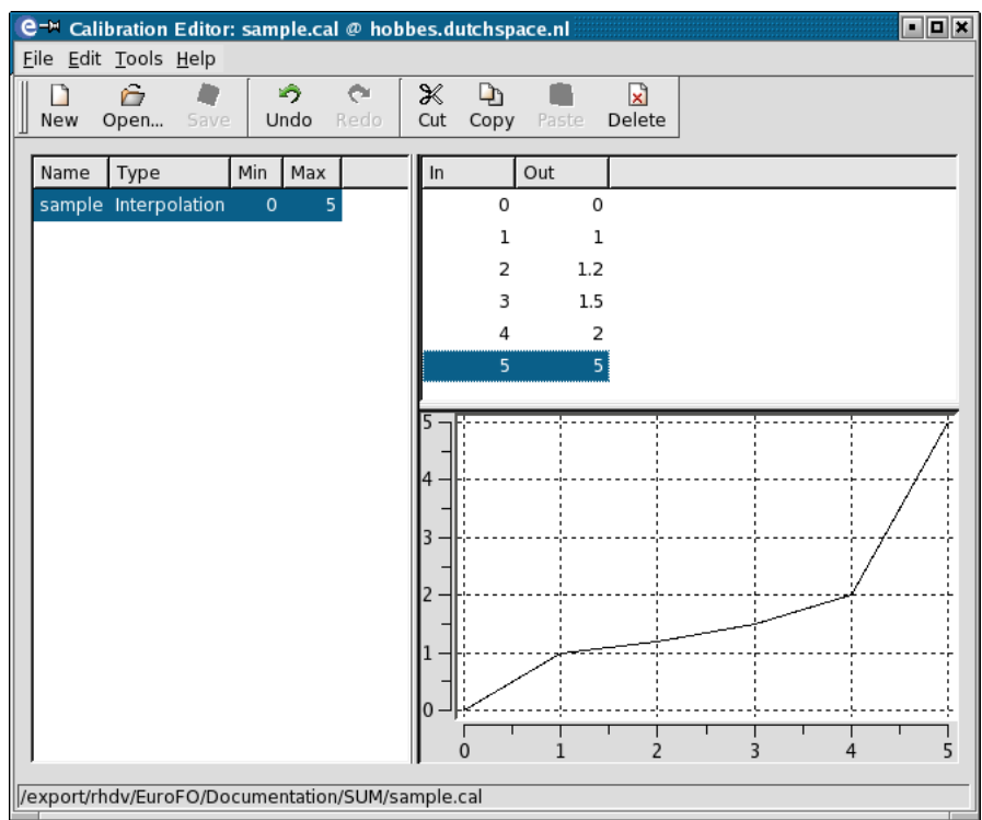
Figure 9.2: Calibration Editor
