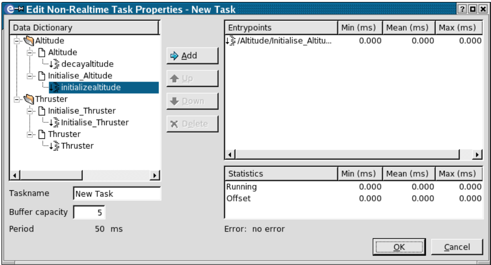
Figure 10.3: Non Real-time Task Dialog
