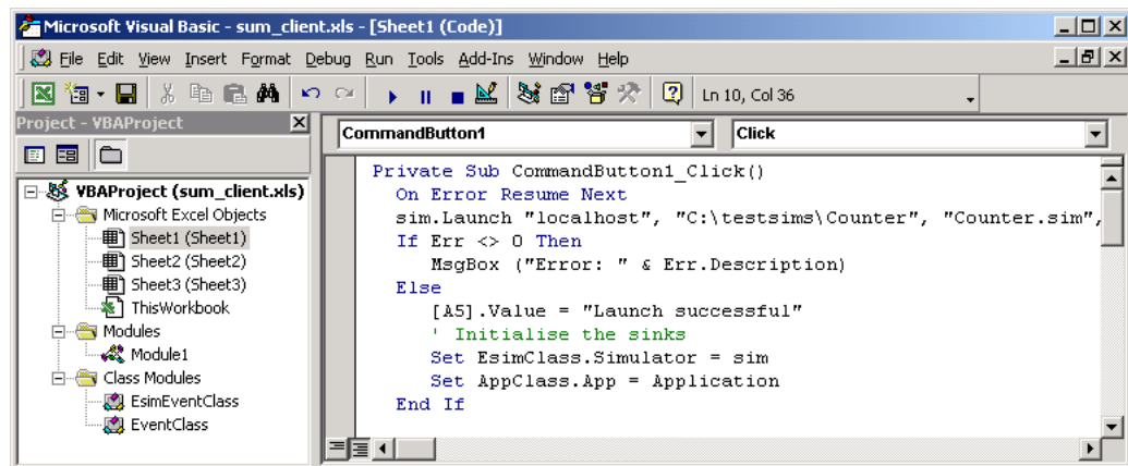
Figure 24.8: Setting the AppClass.App
