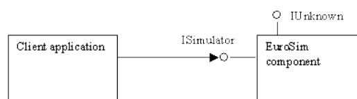
Figure 24.4: Client calling methods on the ISimulator interface
