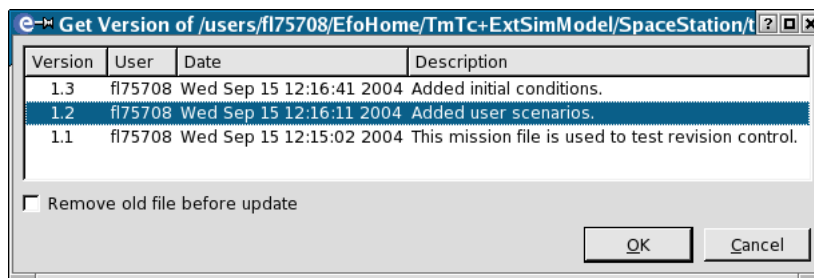
Figure 3.2: Get Version
