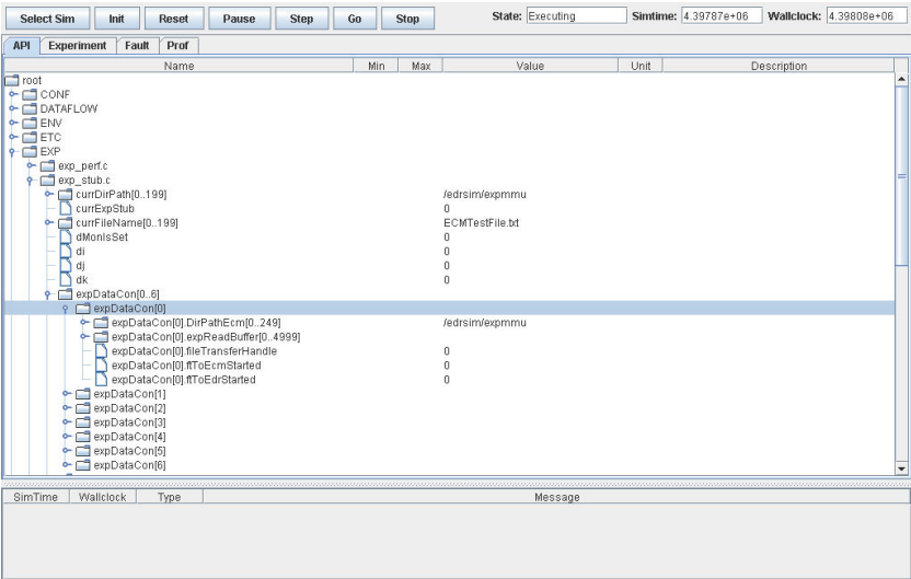
Figure 25.9: API tab
