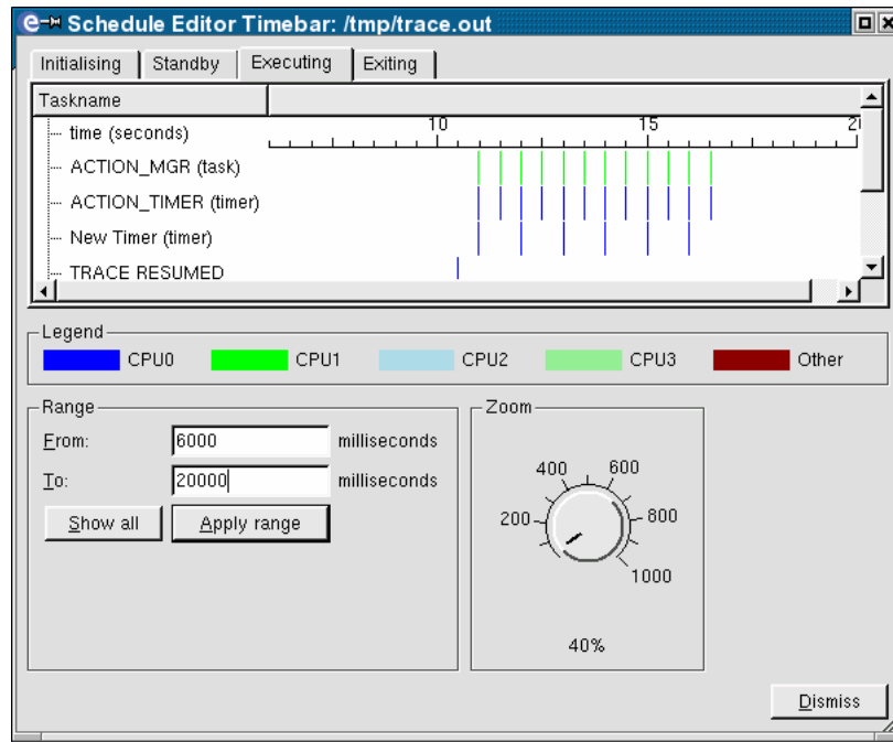
Figure 10.13: Timebar View
