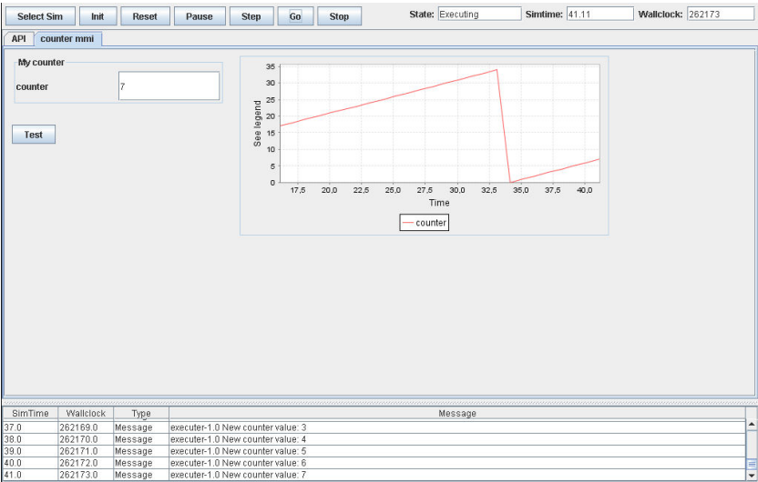
Figure 25.10: MMI tab
