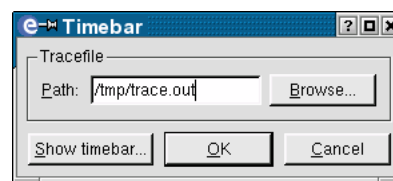
Figure 10.12: Timebar Dialog
