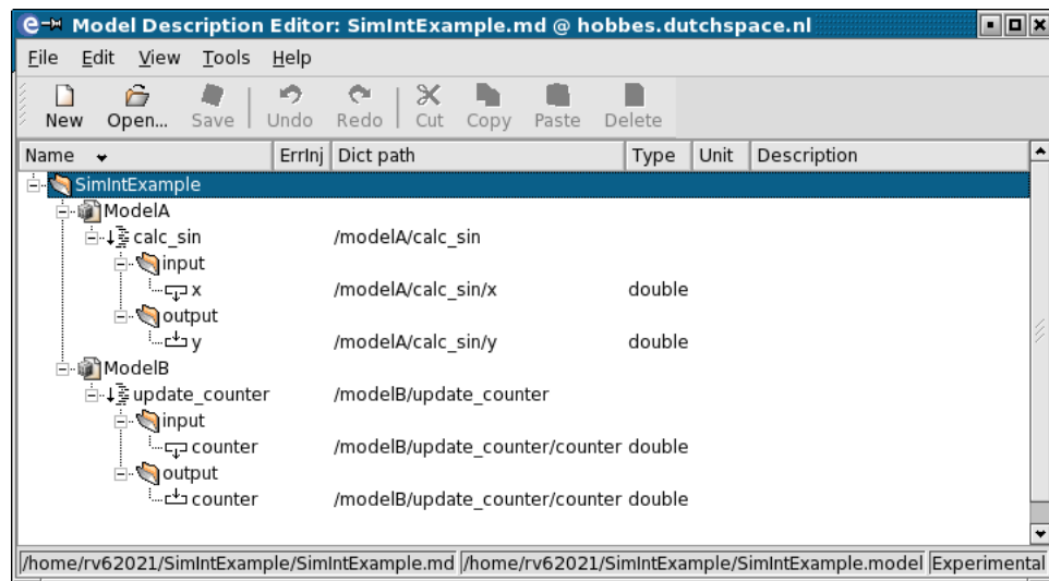
Figure 7.2: Example model description tree
