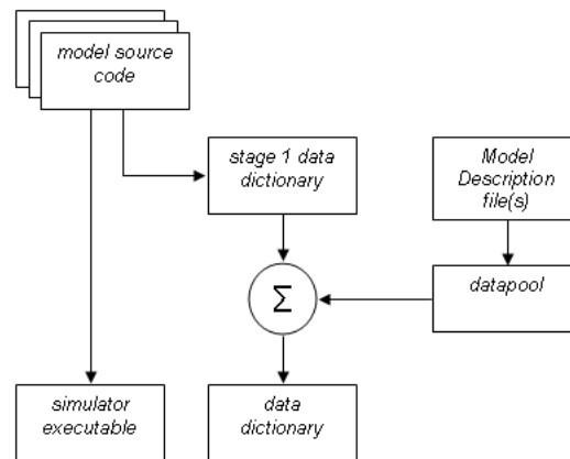
Figure 22.8: Build process steps
