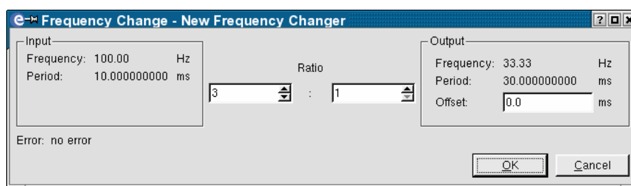
Figure 10.5: Frequency Change Dialog
