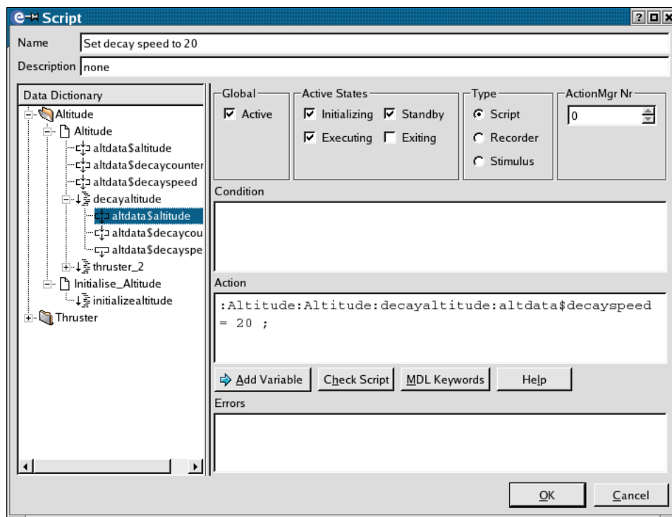
Figure 11.19: The Script Action Editor
