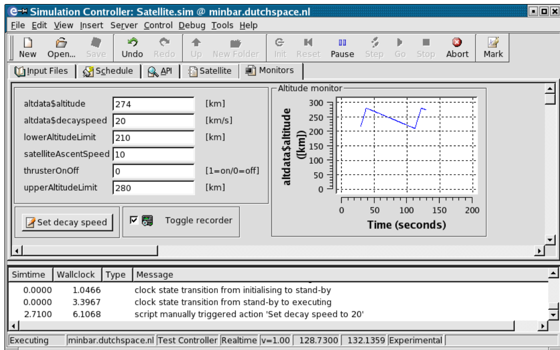
Figure 11.22: The MMI tab page
