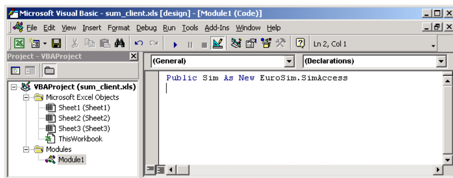
Figure 24.2: Declare an instance of the interface
