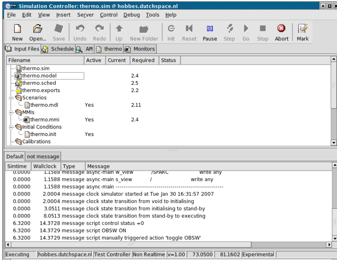
Figure 11.25: The Simulation Controller with message tabs
