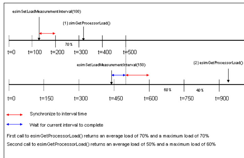
Figure D.1: Example of using the processor load functions
