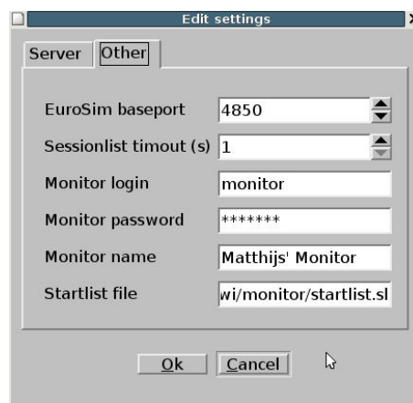
Figure 25.4: The Monitor Settings (second tab)
