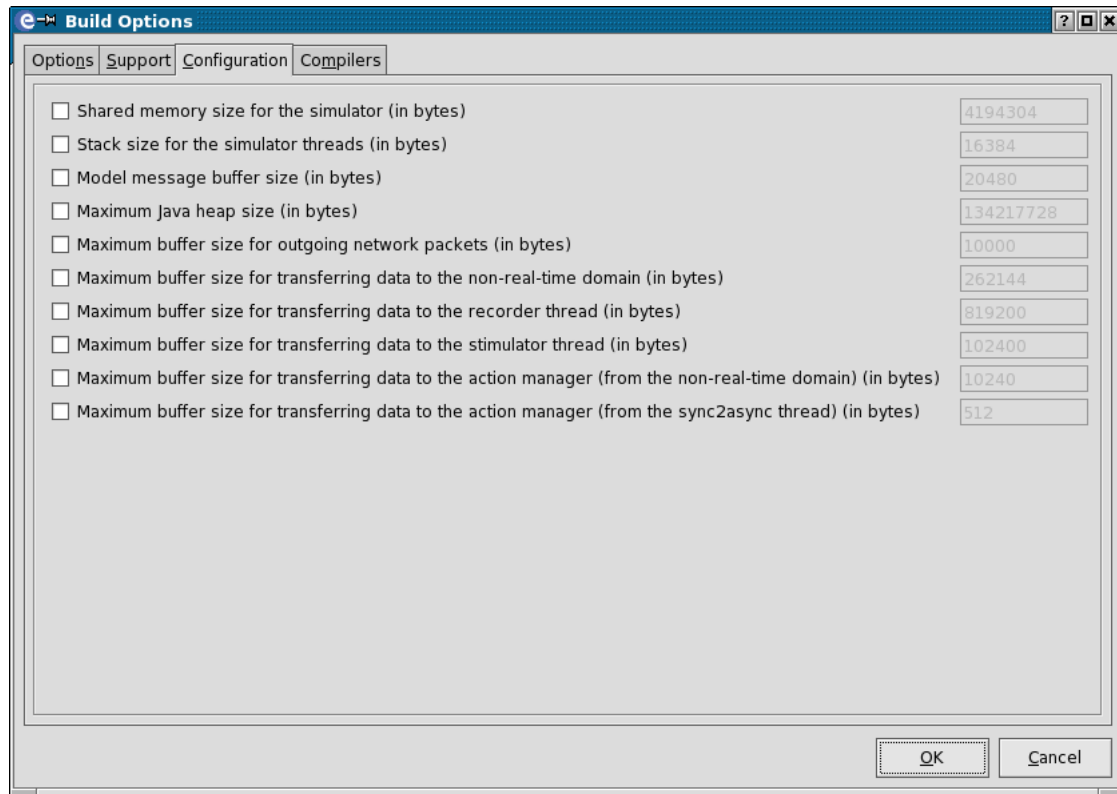
Figure 6.6: Model Build Options dialog: Configuration tab page
