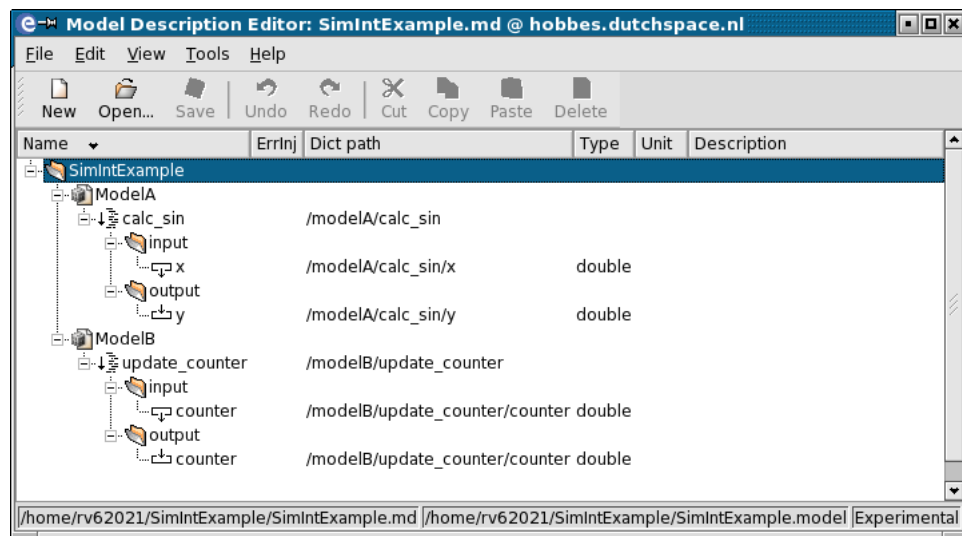
Figure 22.2: Model Description Editor
