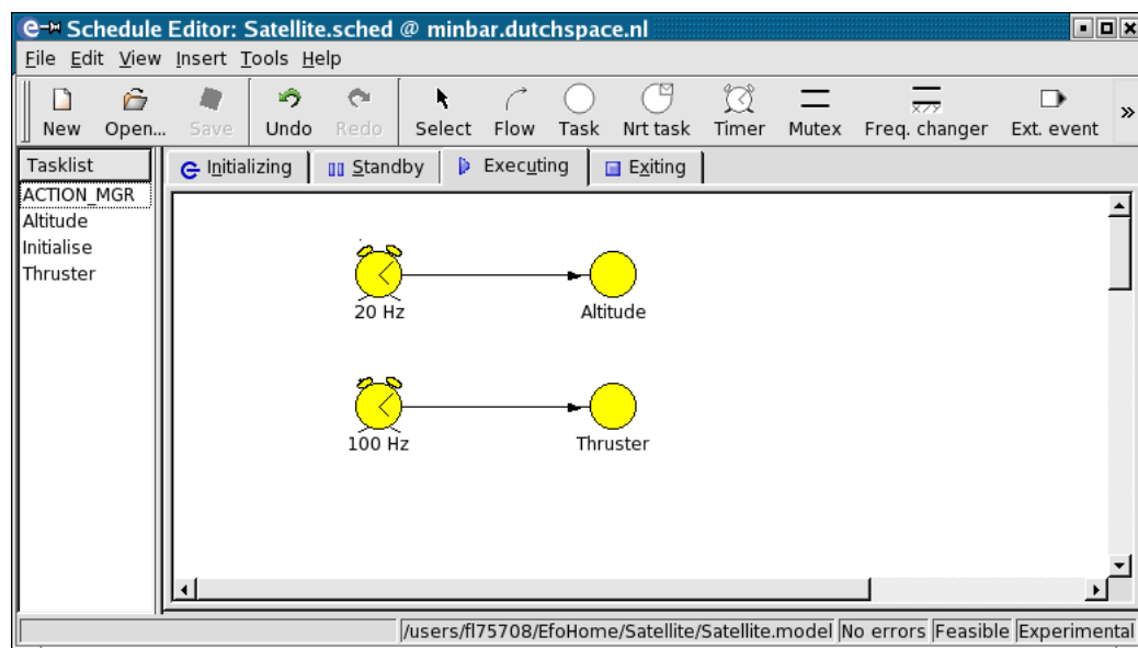
Figure 10.1: Schedule Editor window
