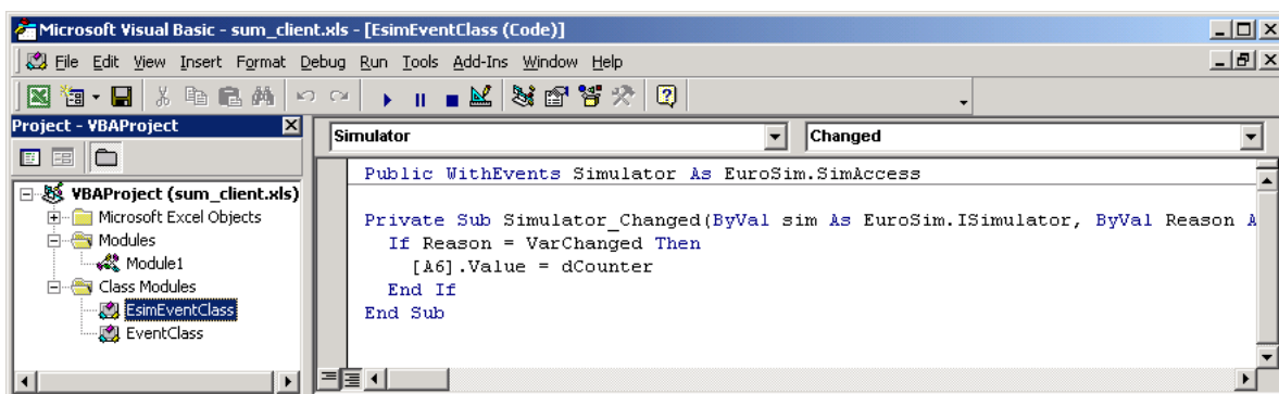
Figure 24.6: Creating an event handler
