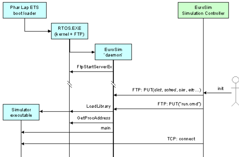
Figure Q.1: Message Sequence Diagram for starting the simulator on a Phar Lap ETS system.
