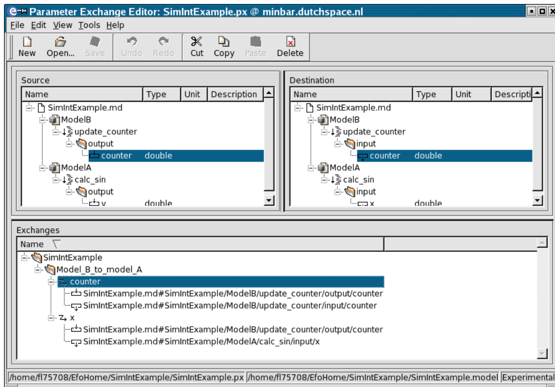
Figure 22.3: Parameter Exchange Editor
