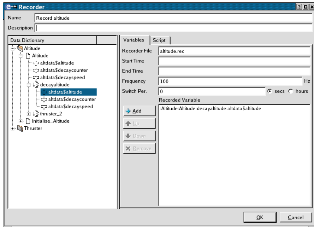
Figure 11.20: The Recorder Action Editor
