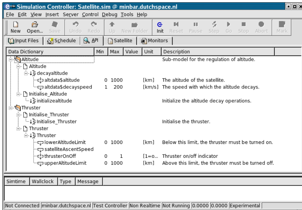
Figure 11.15: The API tab page
