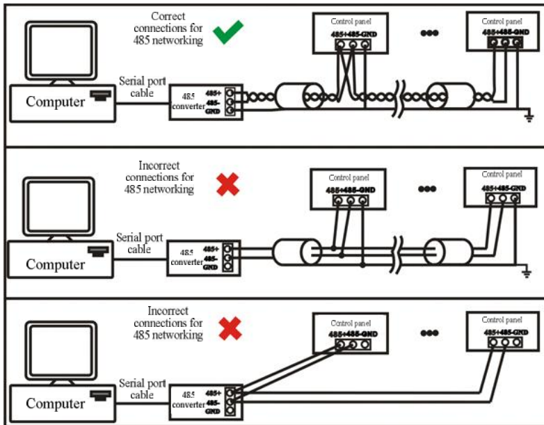
Figure 4-2 RS485 Communication System Networking
