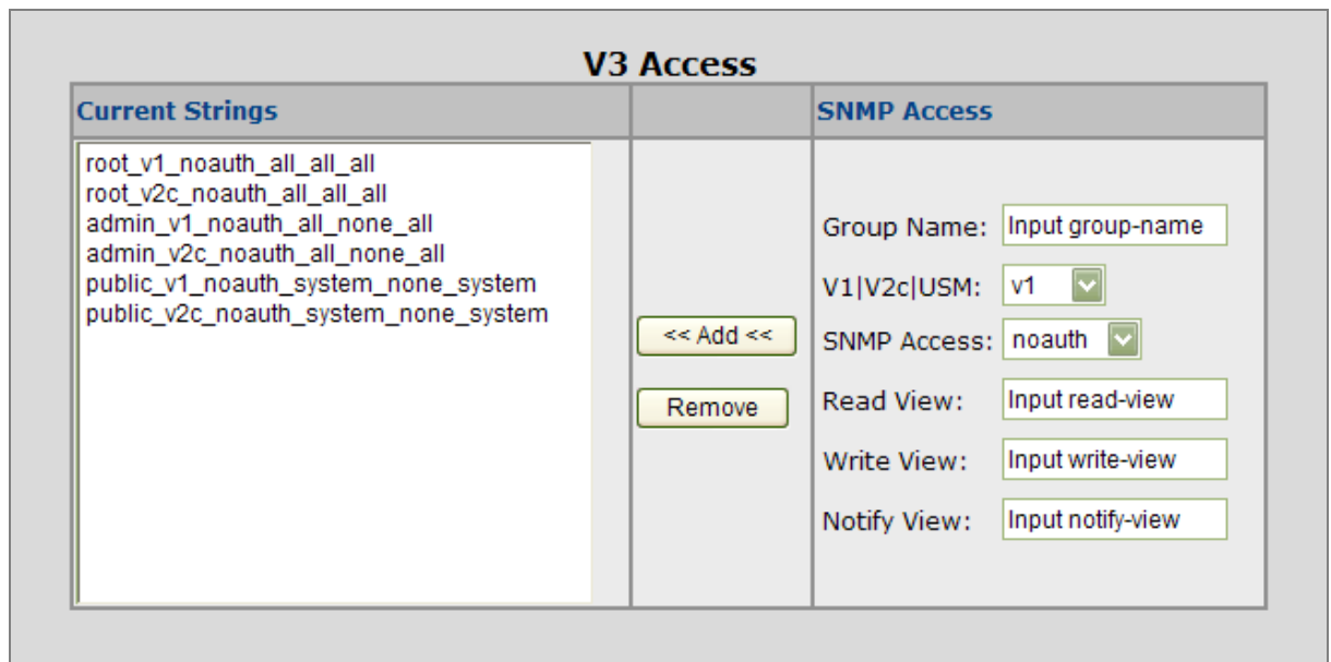
Figure 32: SNMP configuration interface
