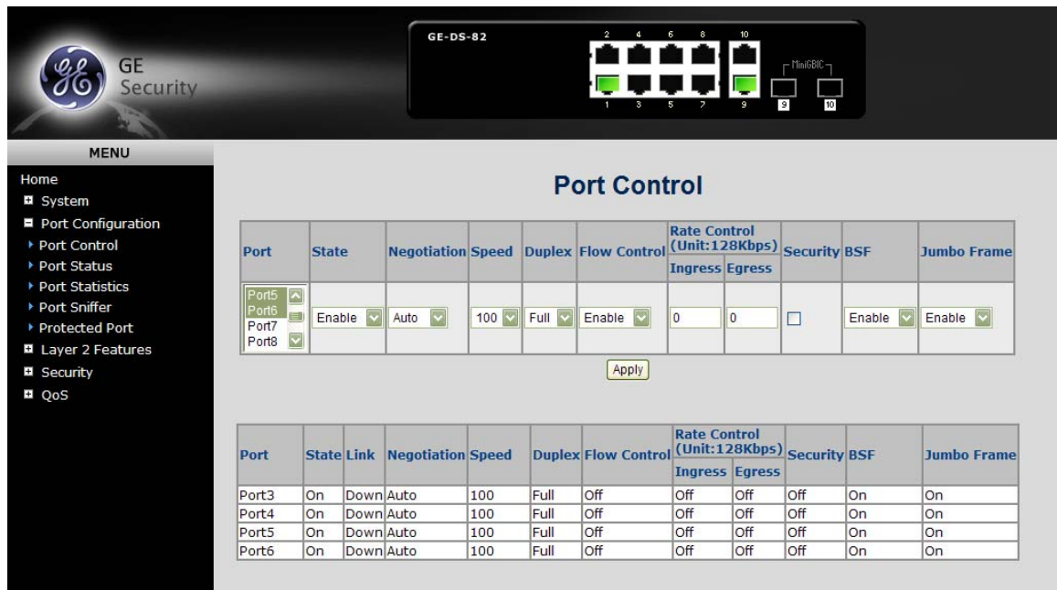
Figure 21: Port Control page
