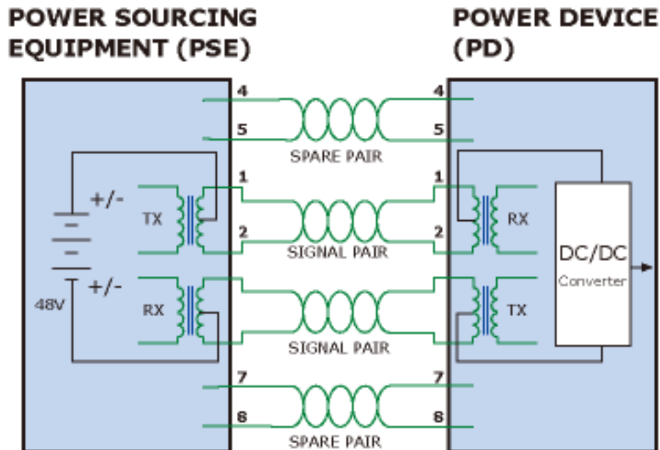
Figure 100: Power Supplied over the Data Pins
