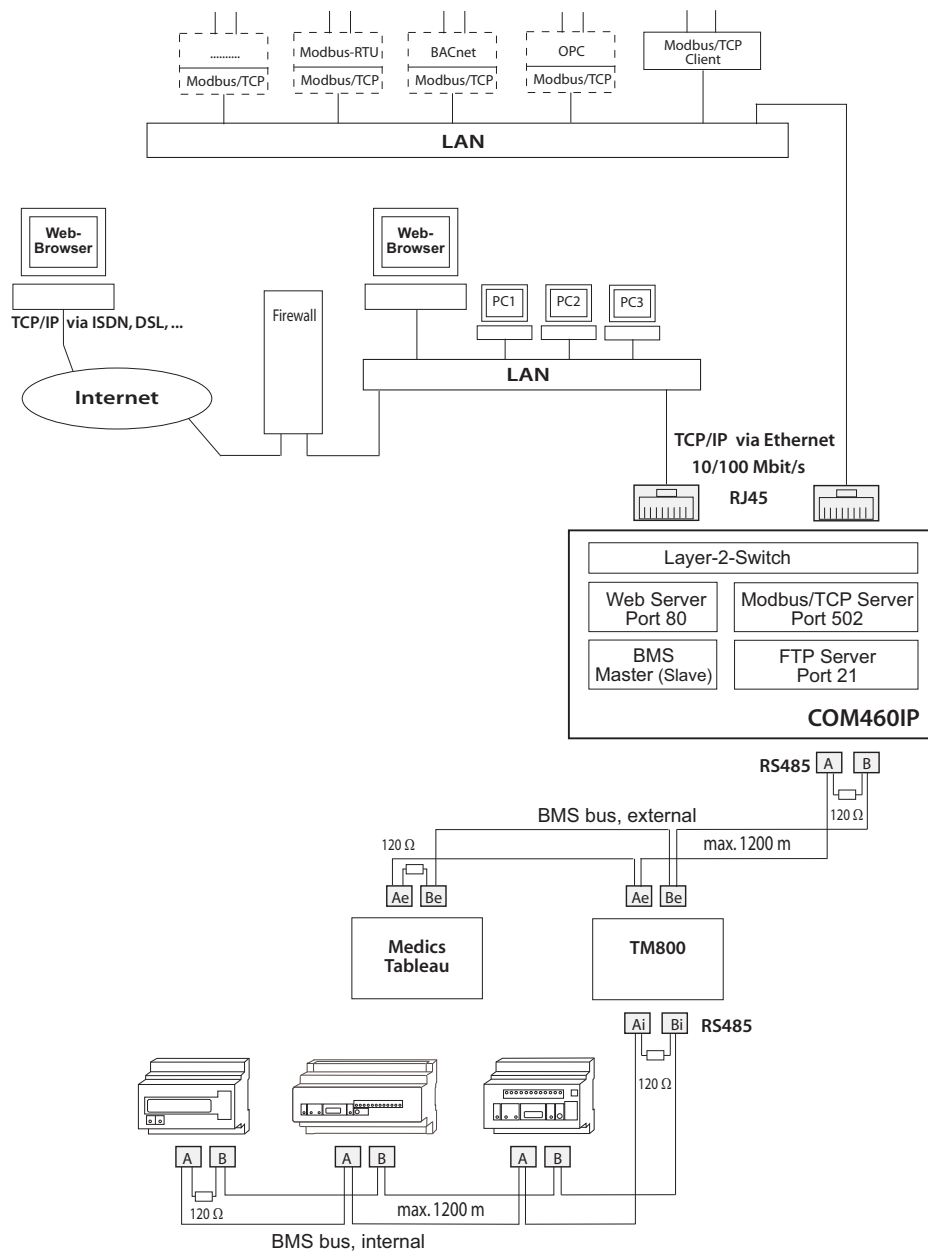
Fig. 4.2: Block diagram of a coupling between an external BMS bus and TCP/IP networks
