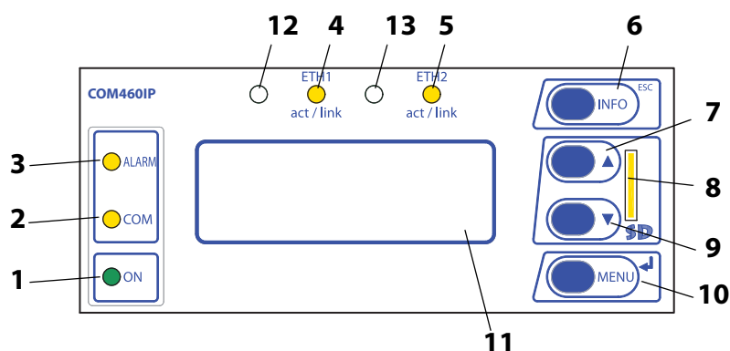
Fig. 6.1: COM460IP front plate
