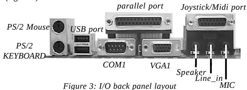
Figure 3: I/O back panel layout
