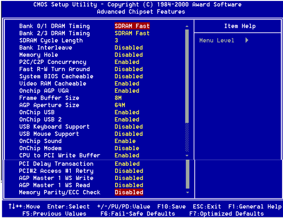
Figure 4: Chipset Features Setup
