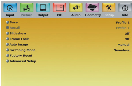
Figure 15: Setup Screen
