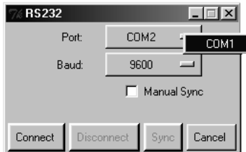
Figure 26: RS-232 Window
