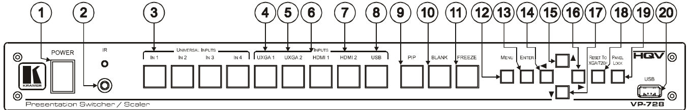
Figure 1: VP-728 Presentation Switcher / Scaler Front Panel
