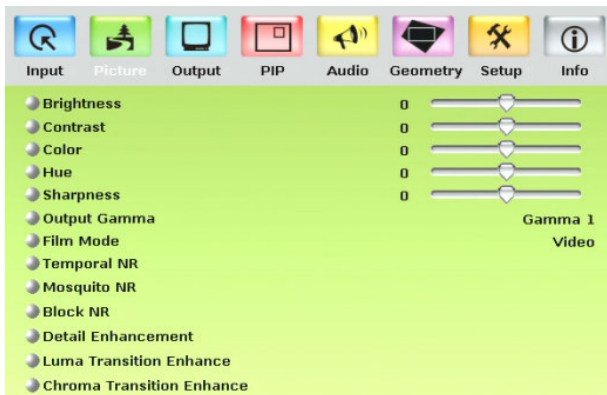
Figure 10: Picture Screen
