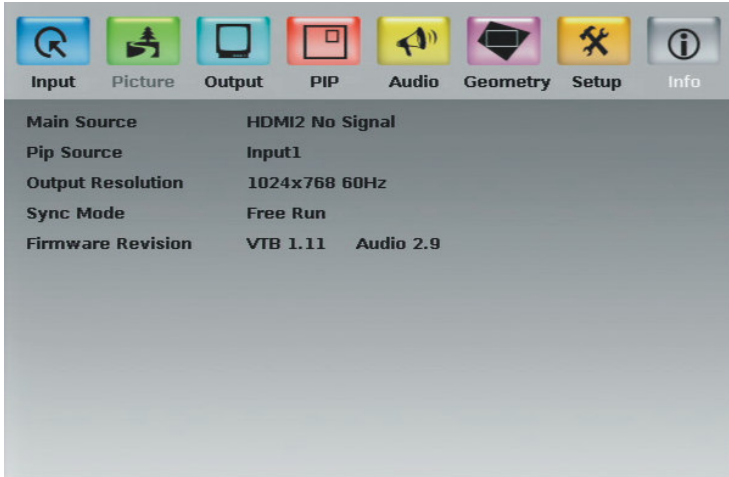
Figure 18: Information Screen
