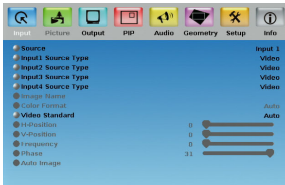
Figure 9: Input Screen
