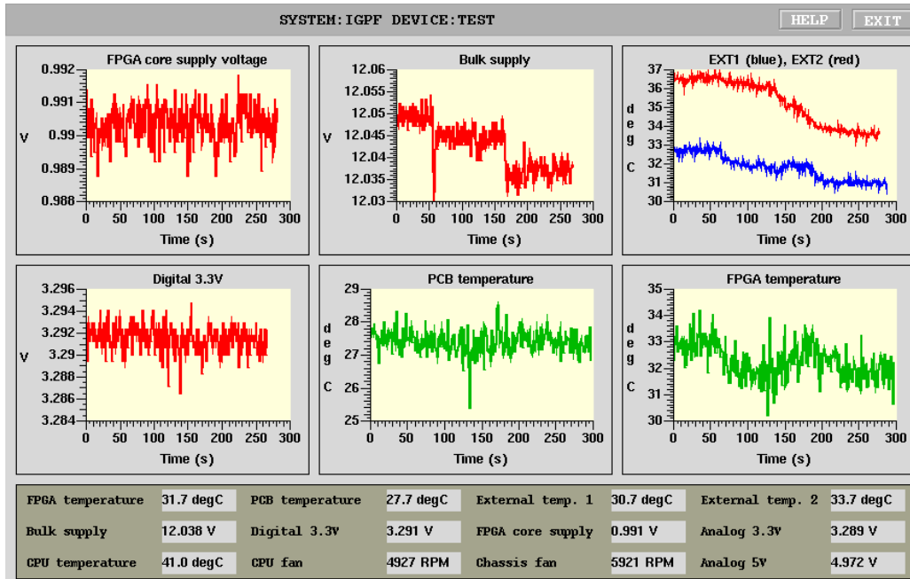
Figure 18: Environmental monitoring panel
