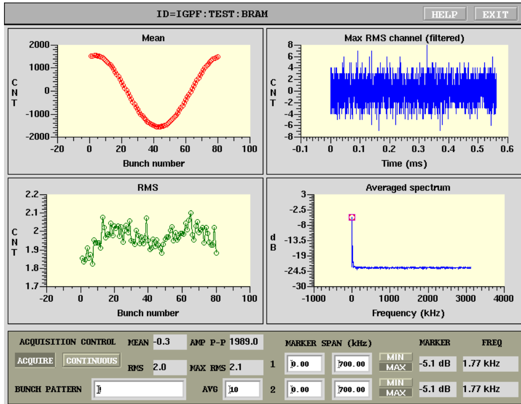
Figure 15: Waveforms panel
