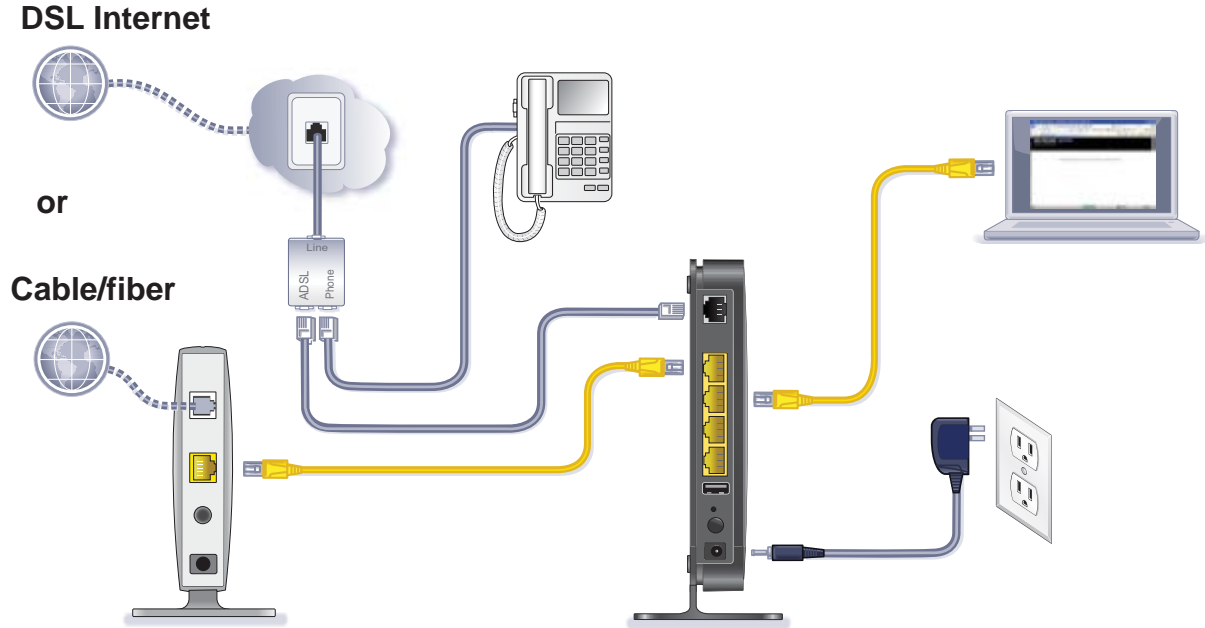
Figure 7. Cable connections
