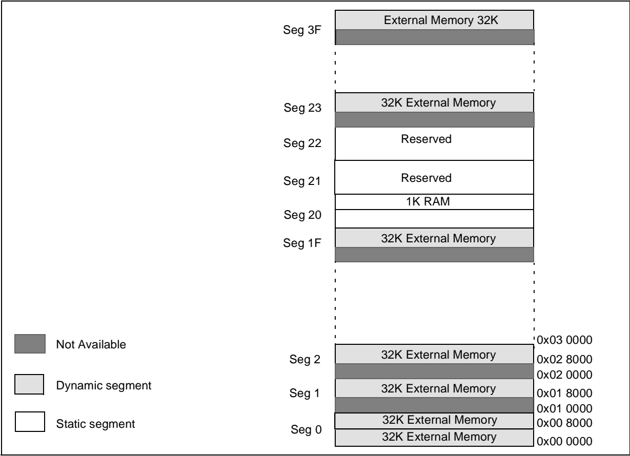
Figure 10. Memory mapping for accessing 2M of external memory with ST90R158
