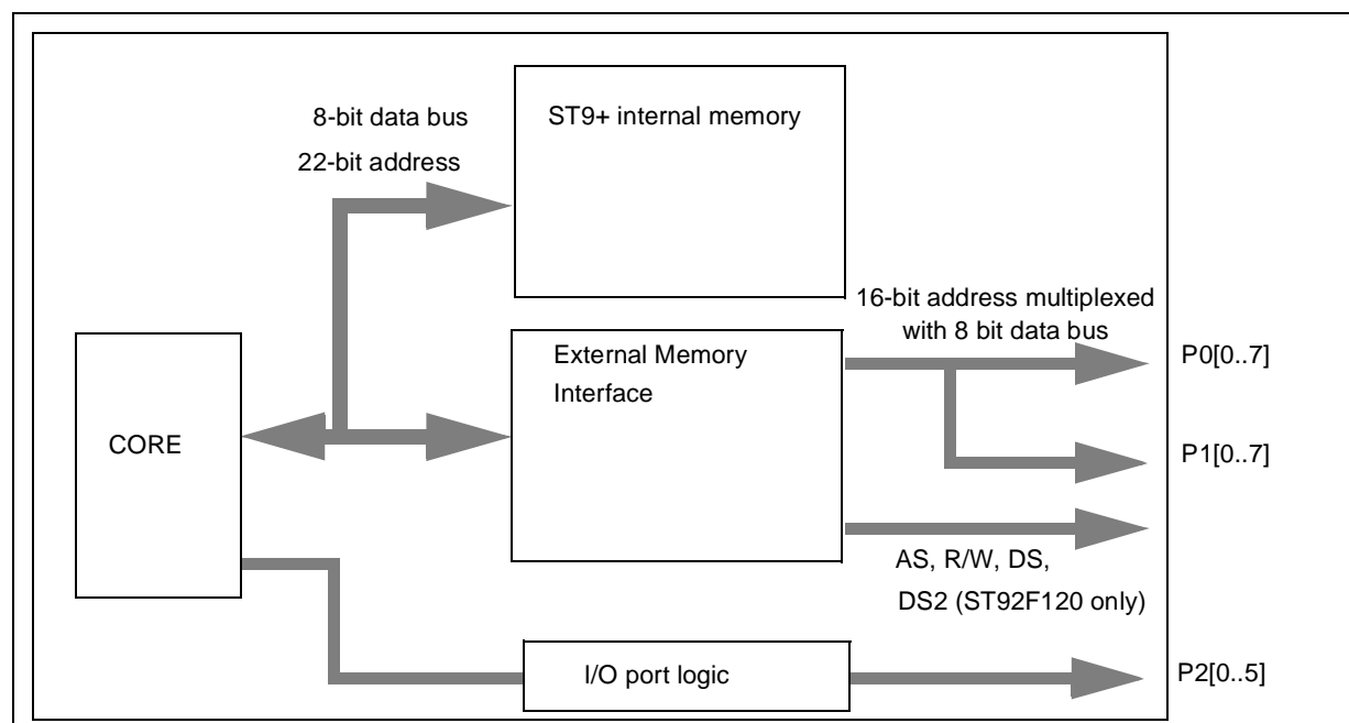
Figure 5. ST9+ Schematic
