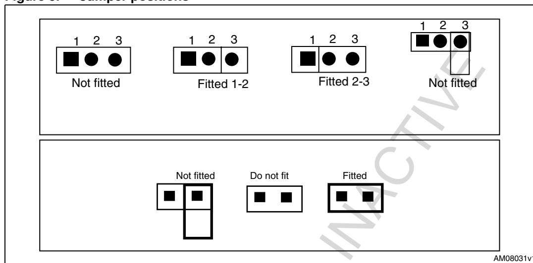
Figure 5. Jumper positions
