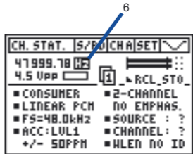
Fig 3-04, PPM setting
