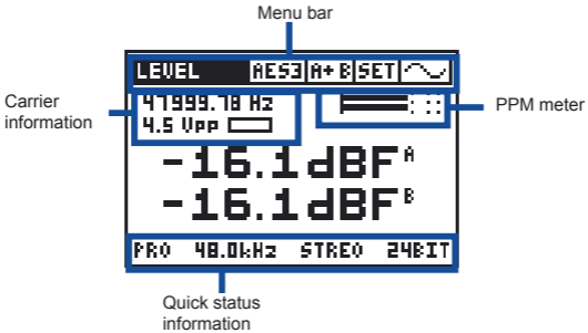
Fig 2-01, Overview display
