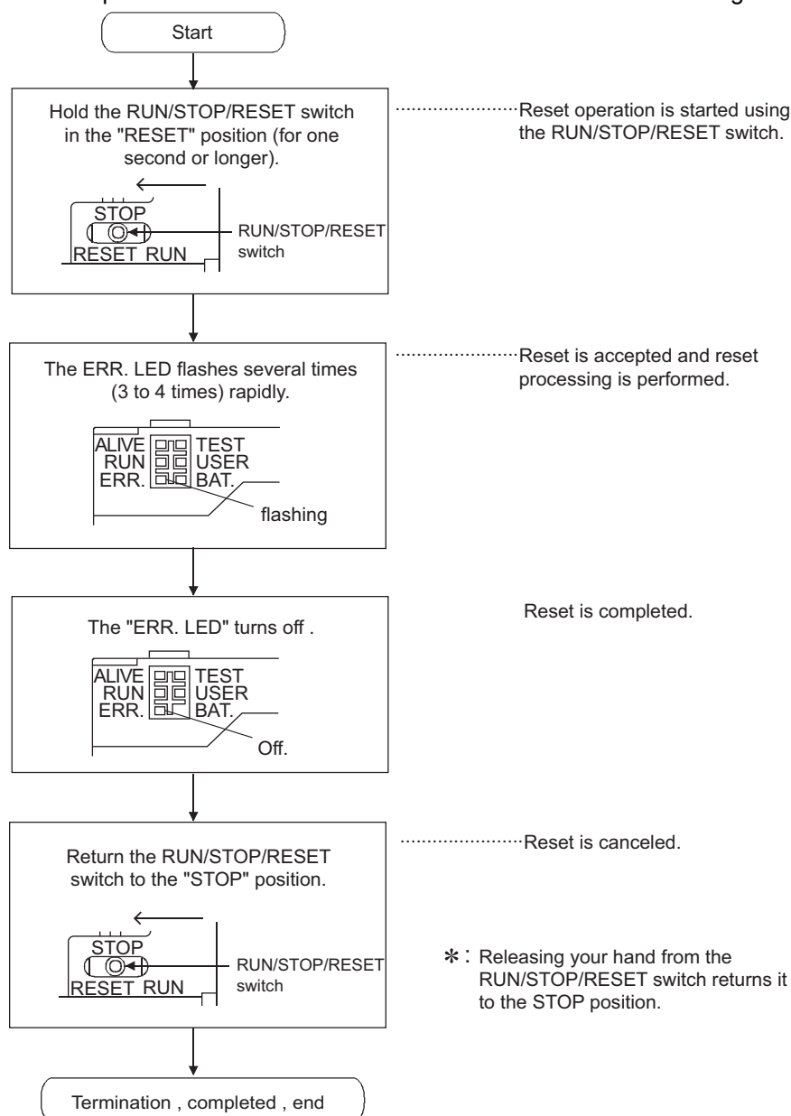
Figure 4.4 Reset Operation
