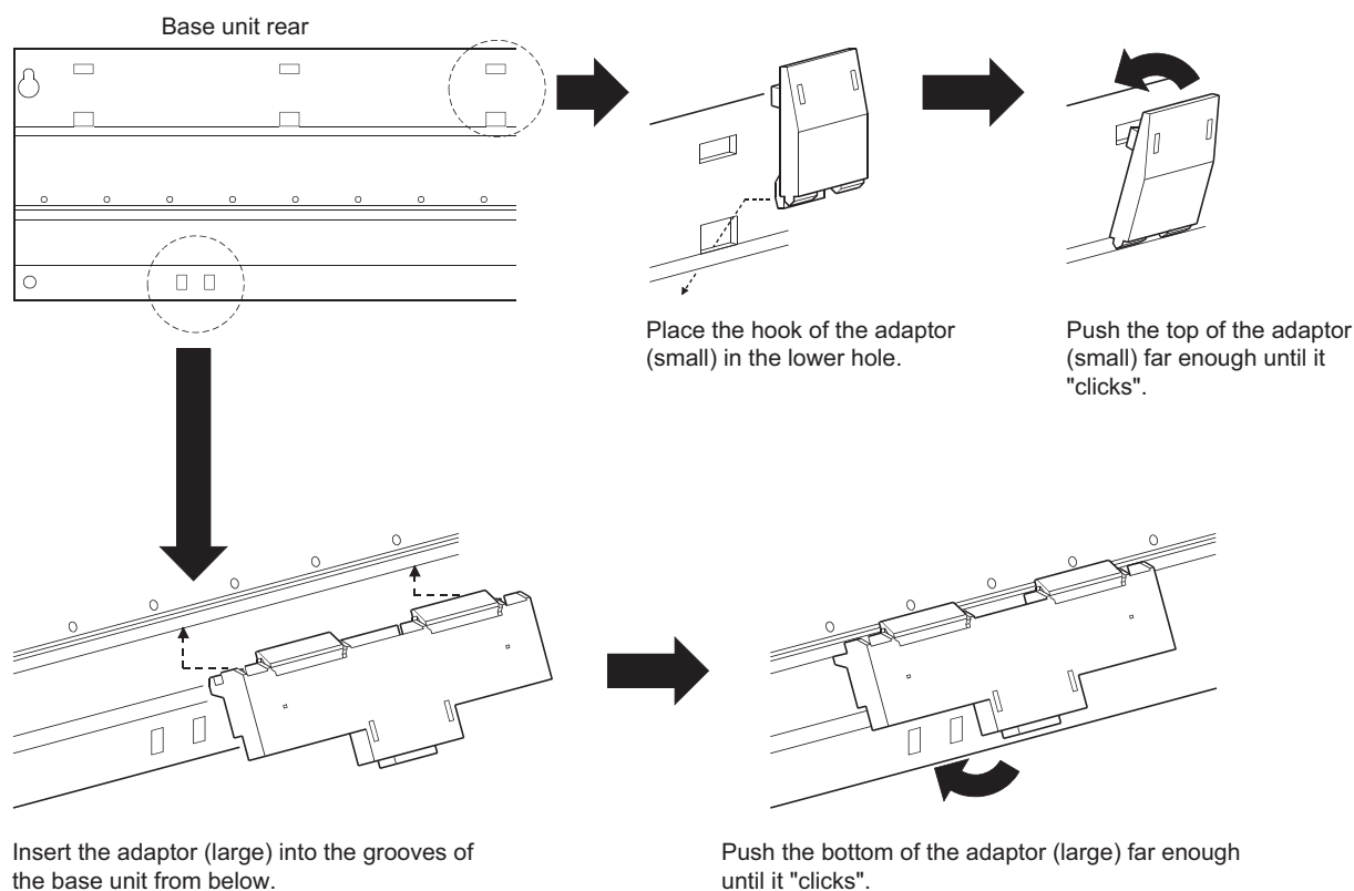
Figure 10.5 Adaptor installation method
