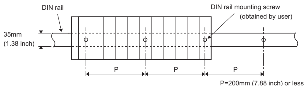
Figure 10.6 DIN rail mounting screw intervals
