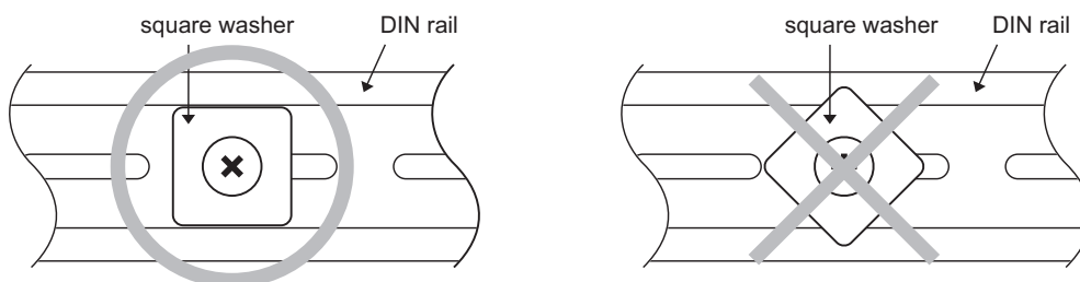
Figure 10.9 Precautions when mounting a square washer
