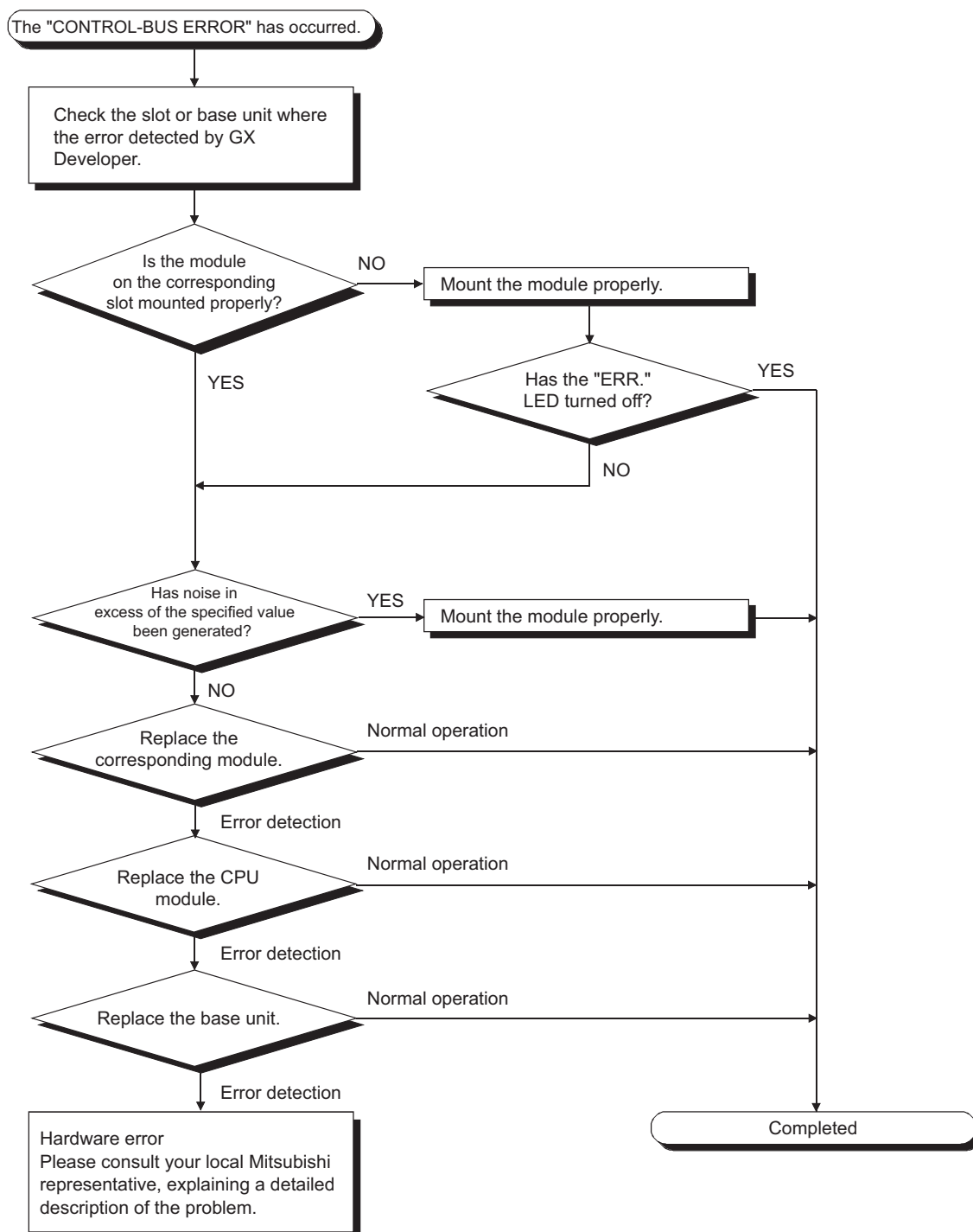
Figure 12.5 Flowchart for when the "ERR." LED is on/flashing
