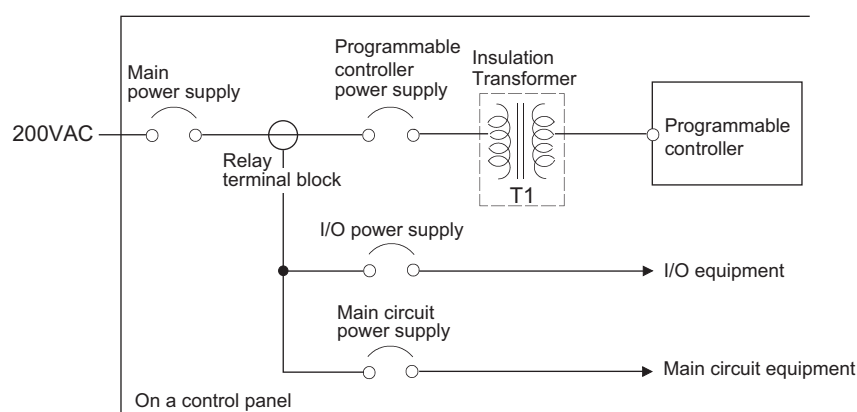
Figure 10.21 Power supply connection diagram
