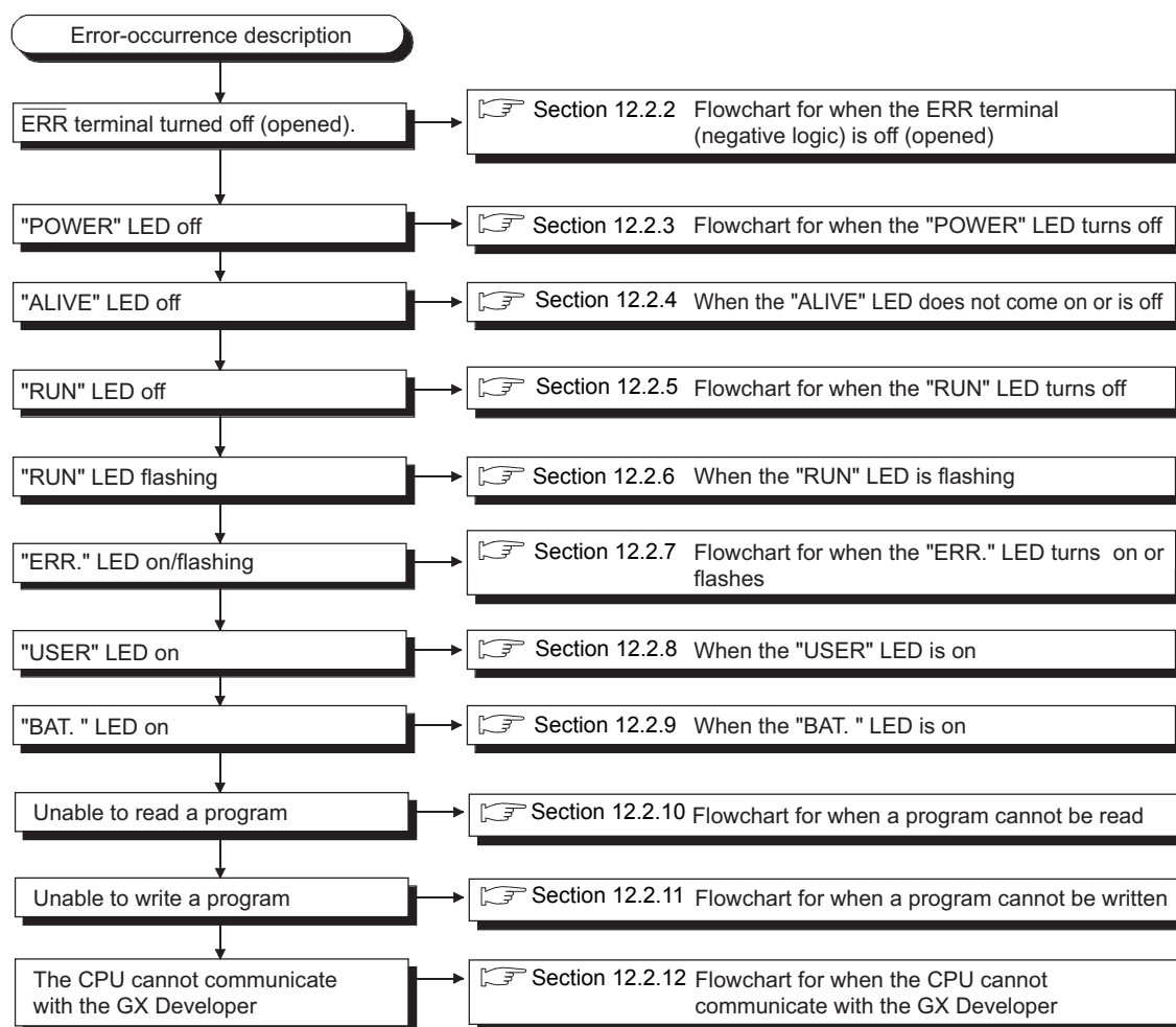
Figure 12.1 Troubleshooting flowchart
