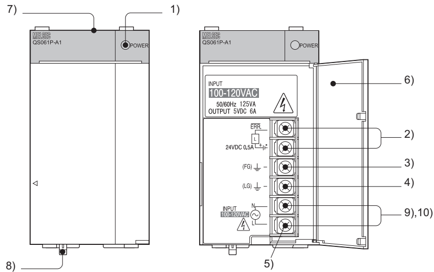
Figure 5.1 Power supply module
