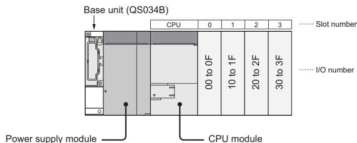
Figure 2.2 System configuration
