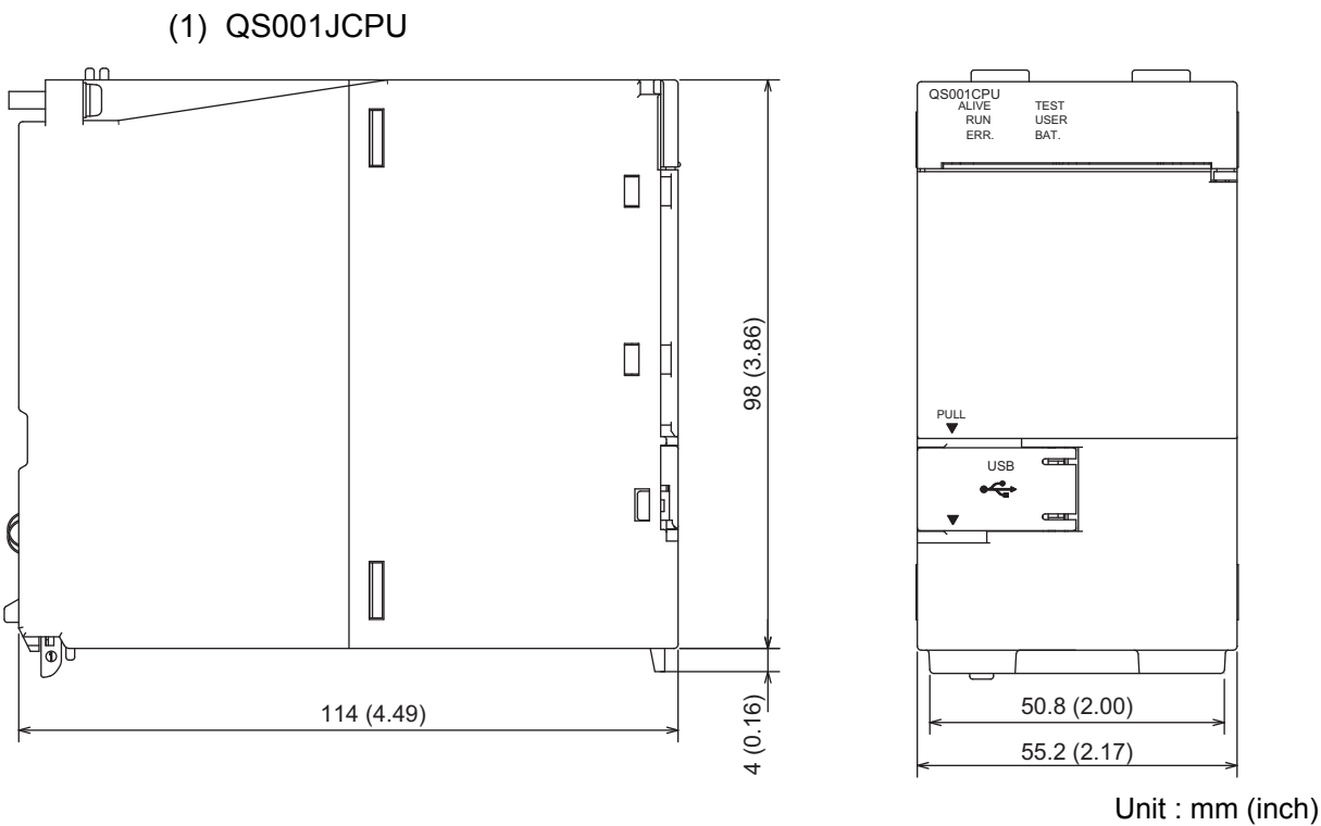
Figure App.1 QS001CPU
