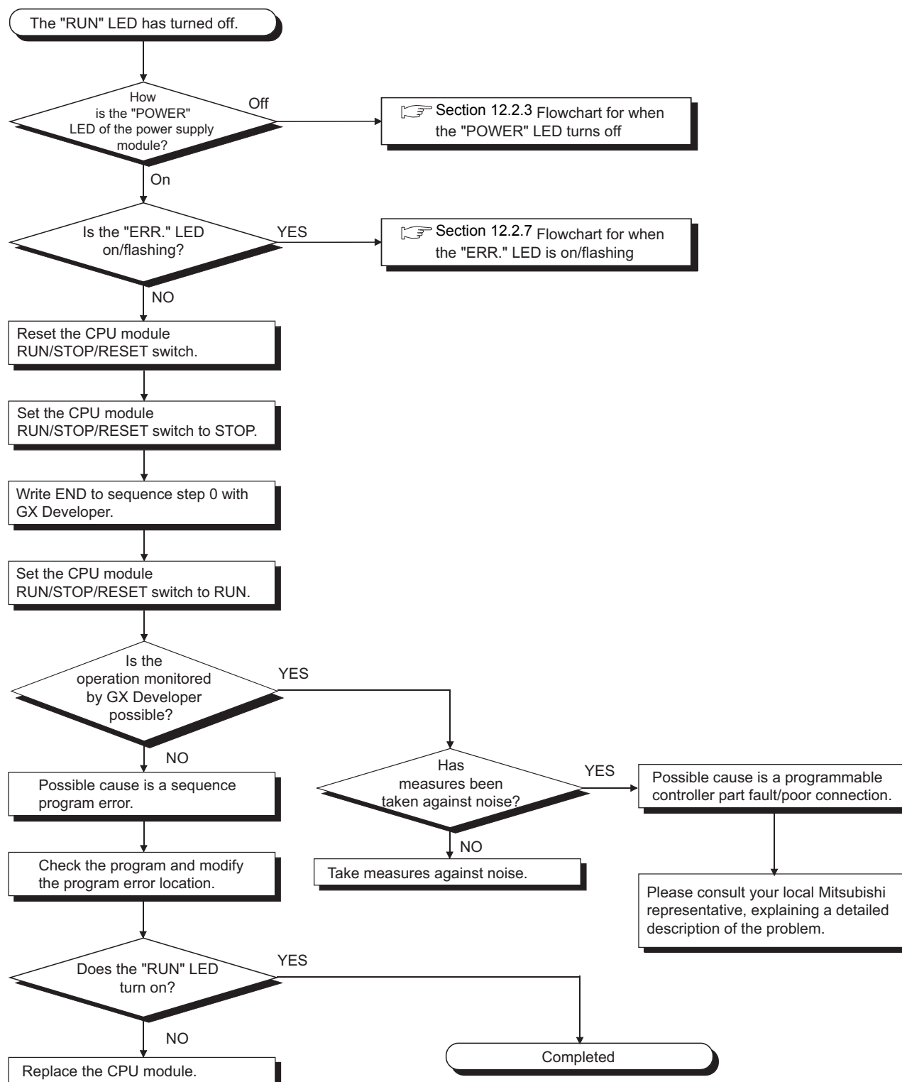
Figure 12.4 Flowchart for when the "RUN" LED turns off
