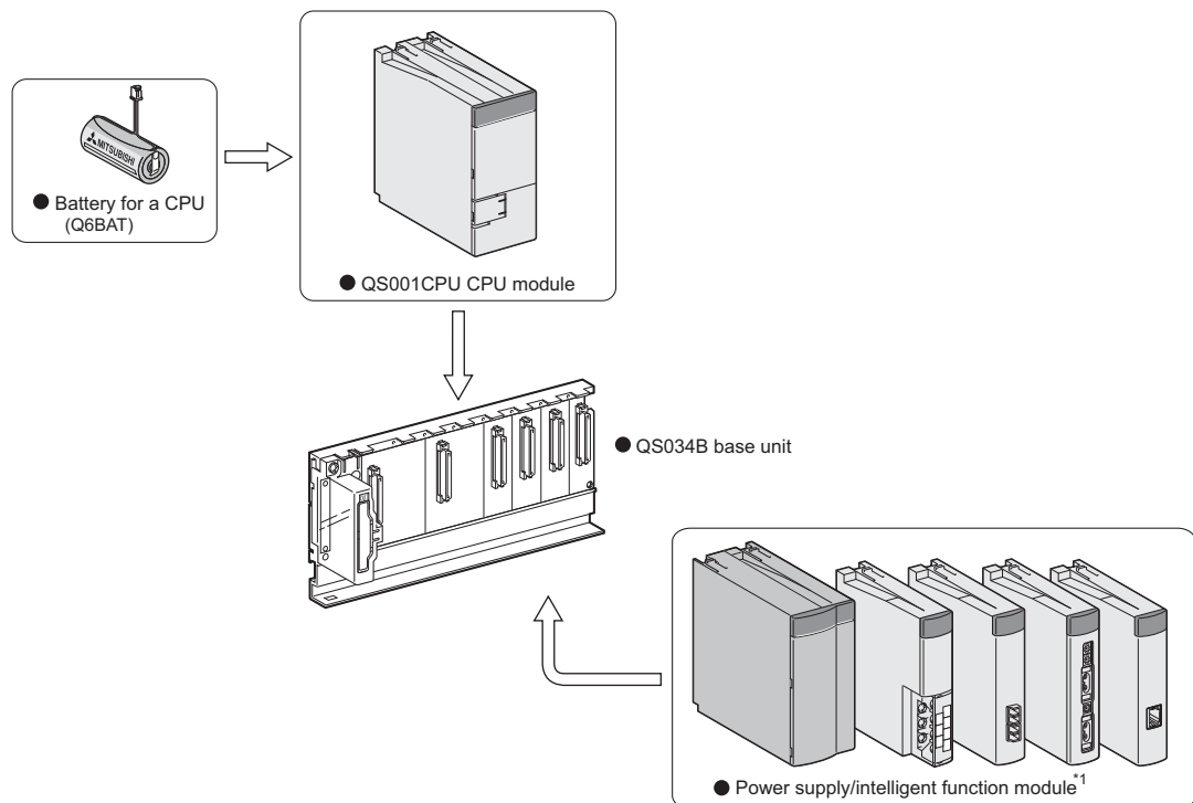
Figure 2.1 System configuration
