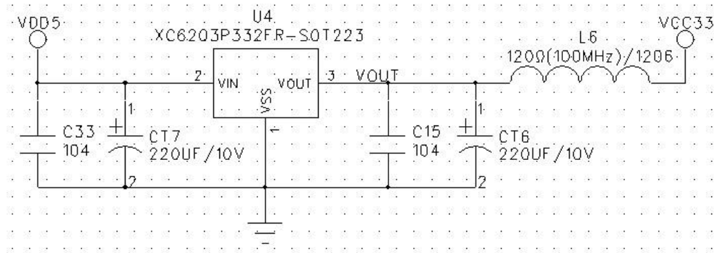
Figure 5-1 Power Reference
