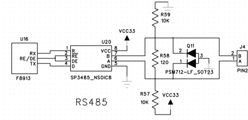
Figure 5-3 F8913D and RS485 connection reference circuit
