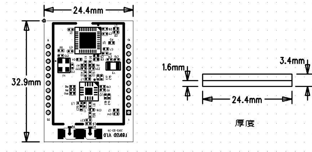
Figure 6-1 Outline Dimension
