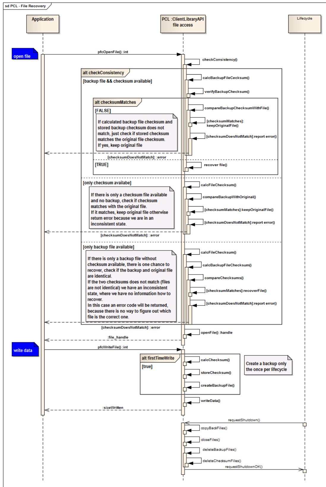
Figure 6 - Recovery Algorithm
