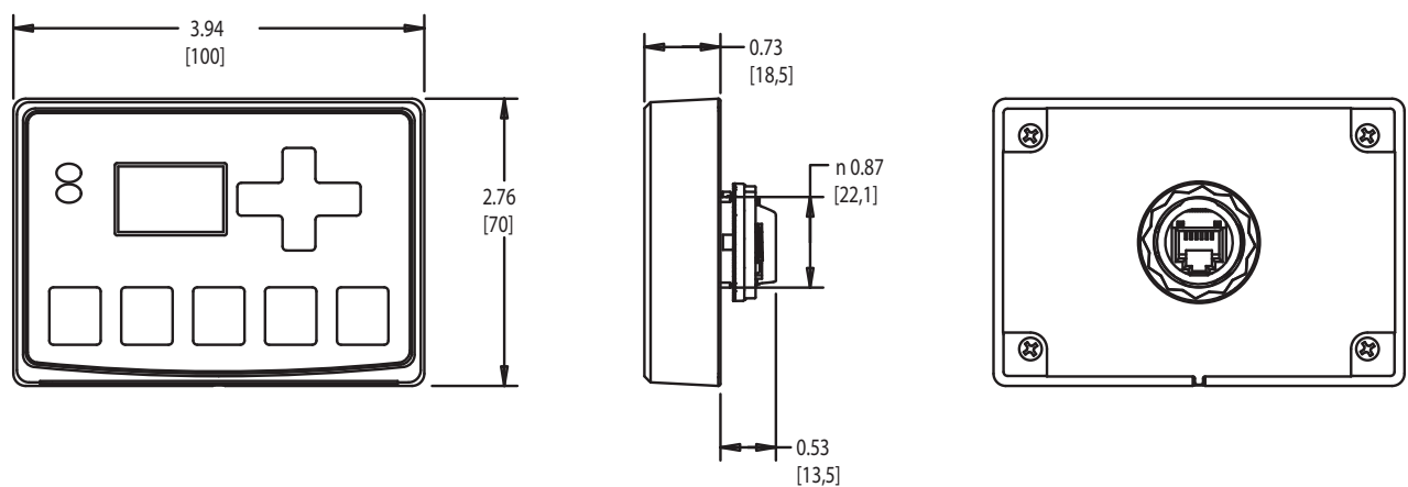
Figure 18 - E300 Starter Diagnostic Station 193-EOS-SDS
