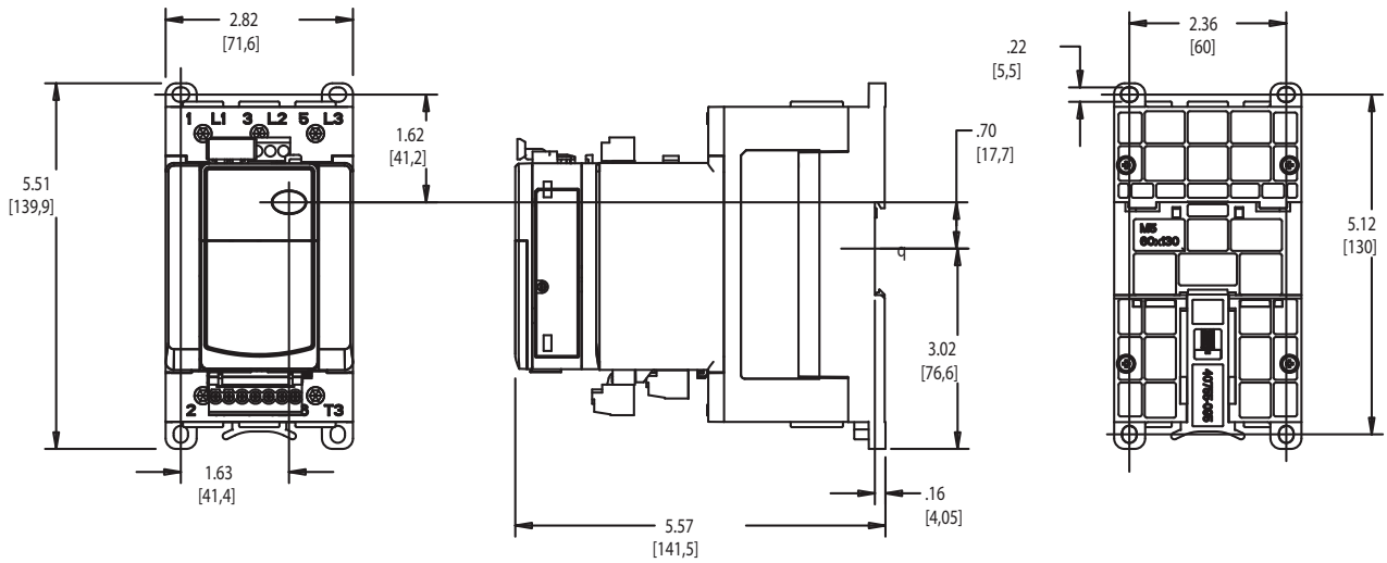
Figure 12 - E300 Overload Relay, 193-ESM-___-100A-E3T, DIN Rail/Panel Mounted
