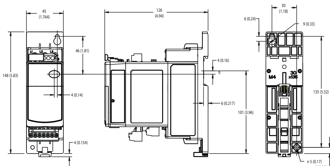
Figure 11 - E300 Overload Relay, 193-ESM-___-30A-E3T and -60A-E3T, DIN Rail/Panel Mounted
