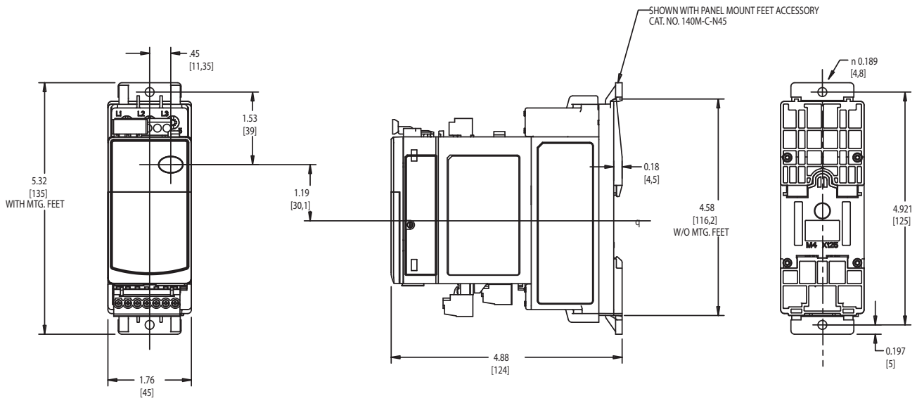
Figure 13 - E300 Overload Relay, 193-ESM-___-30-T and -60A-T, DIN Rail Mounted
