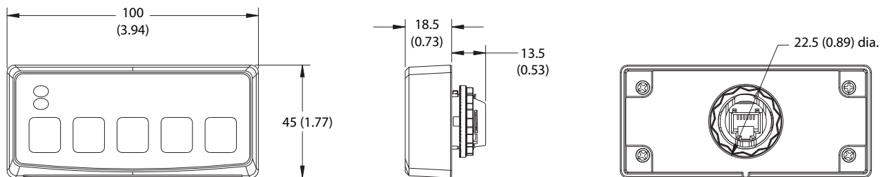
Figure 17 - E300 Starter Control Station 193-EOS-SCS
