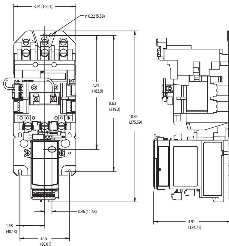
Figure 11 - E300 Overload Relay, 193-ESM-___-30A-E3T and -60A-E3T, DIN Rail/Panel Mounted
