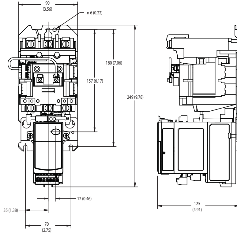
Figure 9 - E300 Overload Relay Mounted on Bulletin 500 NEMA Size 0 and Size 1 Contactor
