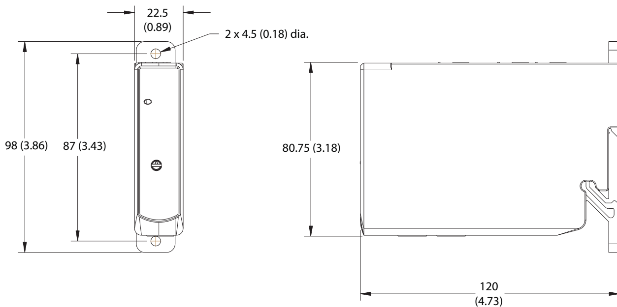
Figure 15 - E300 Analog Expansion Module 193-EXP-AIO-31
