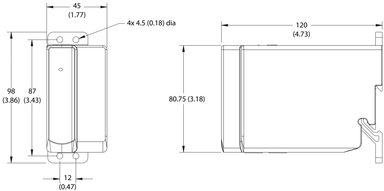
Figure 17 - E300 Starter Control Station 193-EOS-SCS
