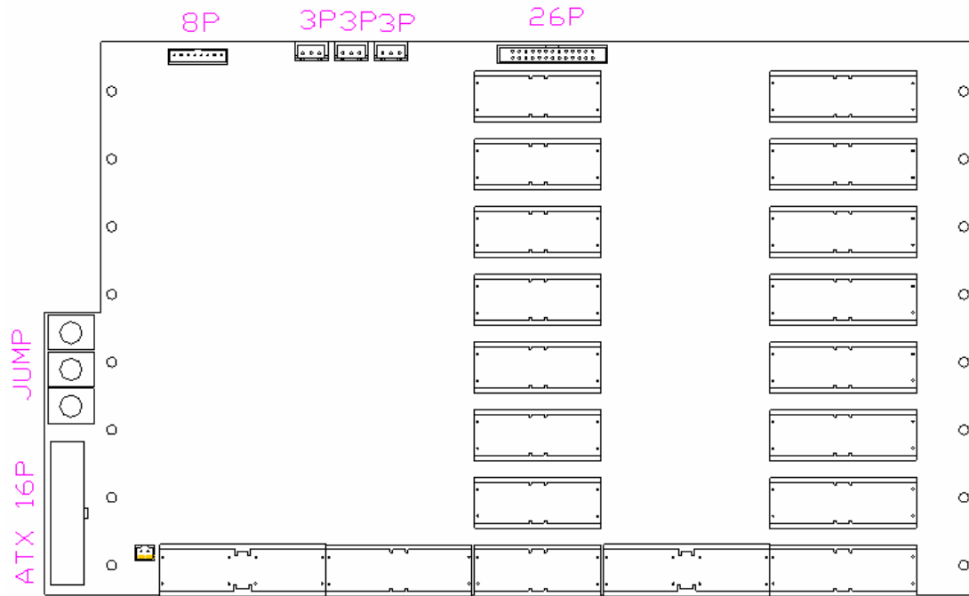
Figure 3-4: The connector and jumper locations on the rear side. (MIC-3038A)
