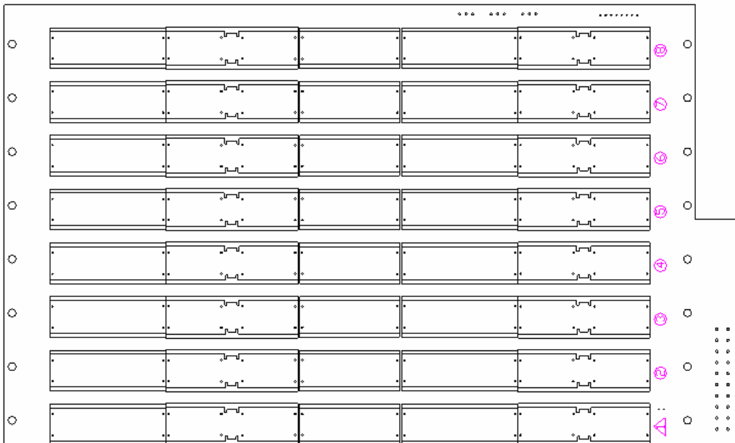
Figure 3-3: The connector and jumper locations on the front side (MIC-3038A)
