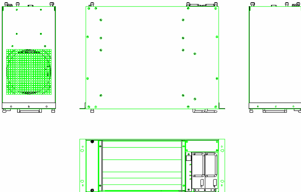
Figure 1-2: Outlook of MIC-3038
