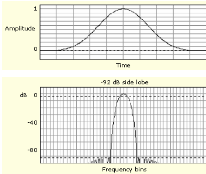
Blackman-Harris window
