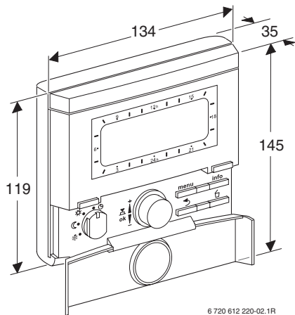
Fig. 1 Unit dimensions with base (accessory)
