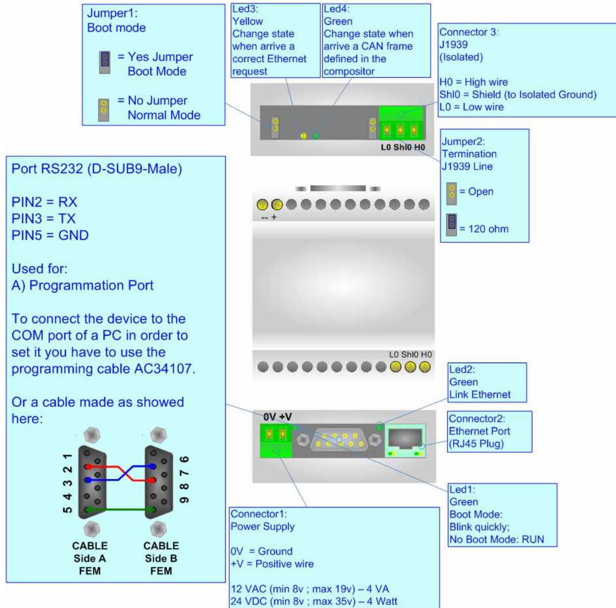
Figure 2: Connection scheme for HD67213M
