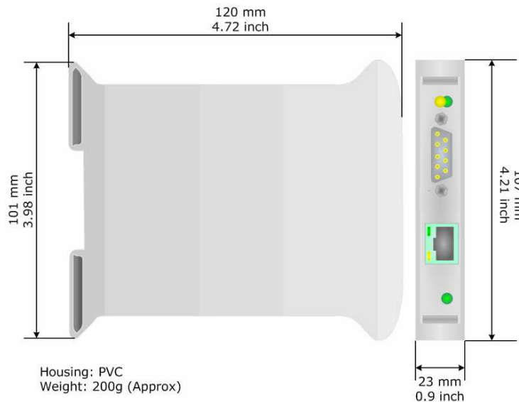
Figure 8: Mechanical dimensions scheme for HD67213
