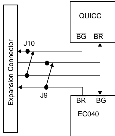
FIGURE 4-1 Arbitration Scheme:
