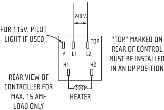
WIRING FOR OPTIONAL 120V/240V CONTROLS
