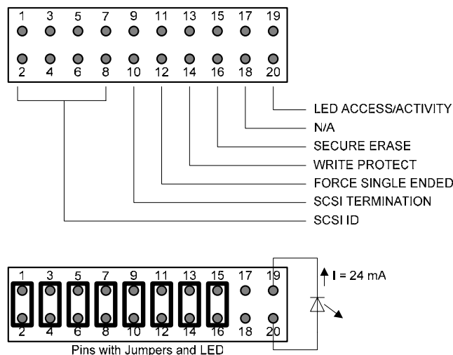
Figure 8: FFD 3.5” Ultra320 SCSI 80-Pin Header Settings
