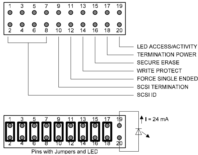
Figure 9: FFD 3.5" Ultra320 SCSI 68-Pin Header Settings
