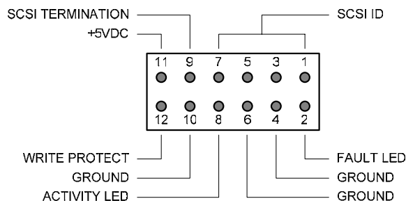
Figure 12: FFD 3.5" Ultra320 SCSI 68-pin Auxiliary Connector Settings
