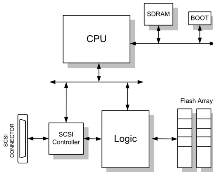
Figure 1: FFD 3.5" Ultra320 SCSI Block Diagram
